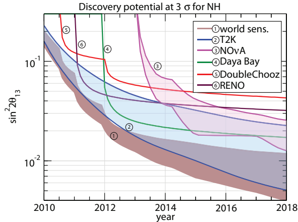
Fig. 2. Evolution of the \theta_{13} discovery potential as a function of time ( 3\sigma C.L.) for NH, showing the global sensitivity reach. The bands for the beams and the global reach reflect the (unknown) true value of \delta . From [15].
