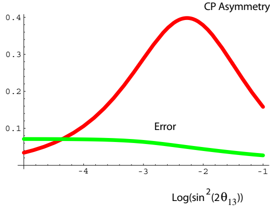
Fig. 1. Magnitude of the CP asymmetry at the first oscillation maximum, for \delta = 1 as a function of the mixing angle \sin^2 2\theta_{13} . The curve marked “error” indicates the dependence of the statistical+systematic error on such a measurement. The curves have been computed for the baseline beta beam option at the fixed energy E_\nu = 0.4 GeV, L = 130 km, statistical + 2% systematic errors. From [6].
