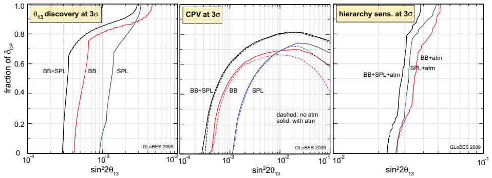
Fig. 3. 3\sigma sensitivities for the beta beam, the SPL super beam and their combination, including or not the atmospheric neutrino data (solid and dashed lines respectively). Computed as a function of the fraction of all possible values of \delta_{CP} . Left panel: sensitivity to \theta_{13} , central panel: sensitivity to leptonic CP violation, right panel: sensitivity to the mass hierarchy, adapted from [43] (courtesy of T. Schwetz).
