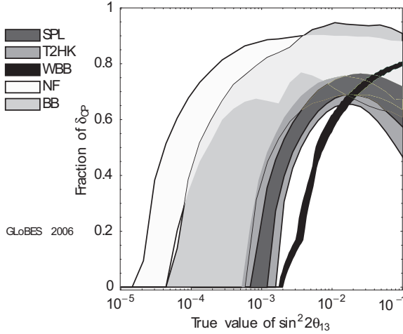
Fig. 4. The discovery reach at 3\sigma level for different facilities in leptonic CP violation sensitivity. The discovery limits are shown as a function of the fraction of all possible values of the true value of the CP phase \delta ('Fraction of \delta_{CP} ') and the true value of \sin^2 2\theta_{13} . The right-hand edges of the bands correspond to the conservative setups while the left-hand edges correspond to the optimized setups. The discovery reach of the SPL super beam is shown as the orange band, that of T2HK as the yellow band, and that of the wide-band beam experiment as the green band. The discovery reach of the beta beam is shown as the light green band and the neutrino factory discovery reach is shown as the blue band. From reference [9].
