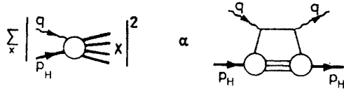
Fig. 2. \sigma(e+H \rightarrow e'+X) given by the parton model motivated by asymptotic freedom
