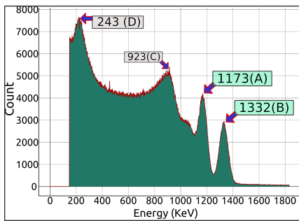
FIG. 2: a) 60 Cobalt gamma spectrum calibrated using the known photopeaks labelled A & B . The Compton edge corresponding to 1173keV photopeak and backscatter peak calculated with this calibration are also labelled as C & D respectively.
