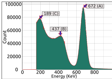
FIG. 3: a) 137 Cesium gamma spectrum showing the photopeak(A), Compton edge(B), and Backscatter Peak(C).
