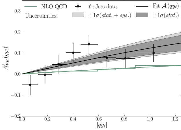
FIG. 7. The binned asymmetry A_{\text{FB}}^{\ell}(qy_{\ell}) after correcting for acceptance, compared to the NLO QCD prediction of POWHEG. The best fit to Eq. (7) for each is shown as the smooth curve of the same color. The dark (light) gray bands indicate the statistical (total) uncertainty on the fit curve to the data.
