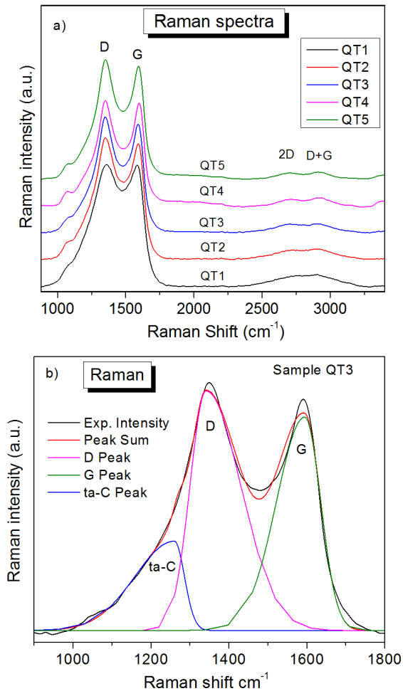
Figure 4: Raman spectra for samples QT1–QT5 in the range from 900 to 3400 \text{cm}^{-1} (a) and deconvoluted Raman spectrum in the range from 900 to 1800 \text{cm}^{-1} for QT3 (b).
