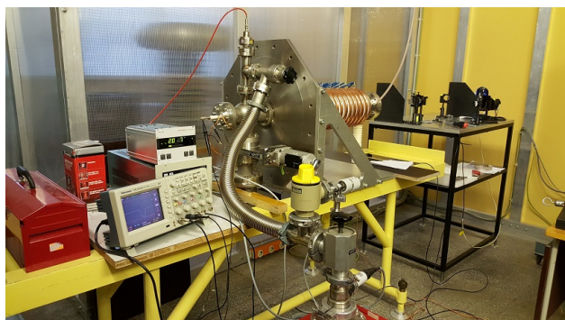
Figure 2: Photoinjector bench setup during the startup.
