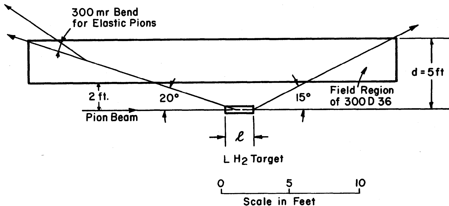
Fig. 2. Relative disposition of target and magnet for backward-scattered particles.
