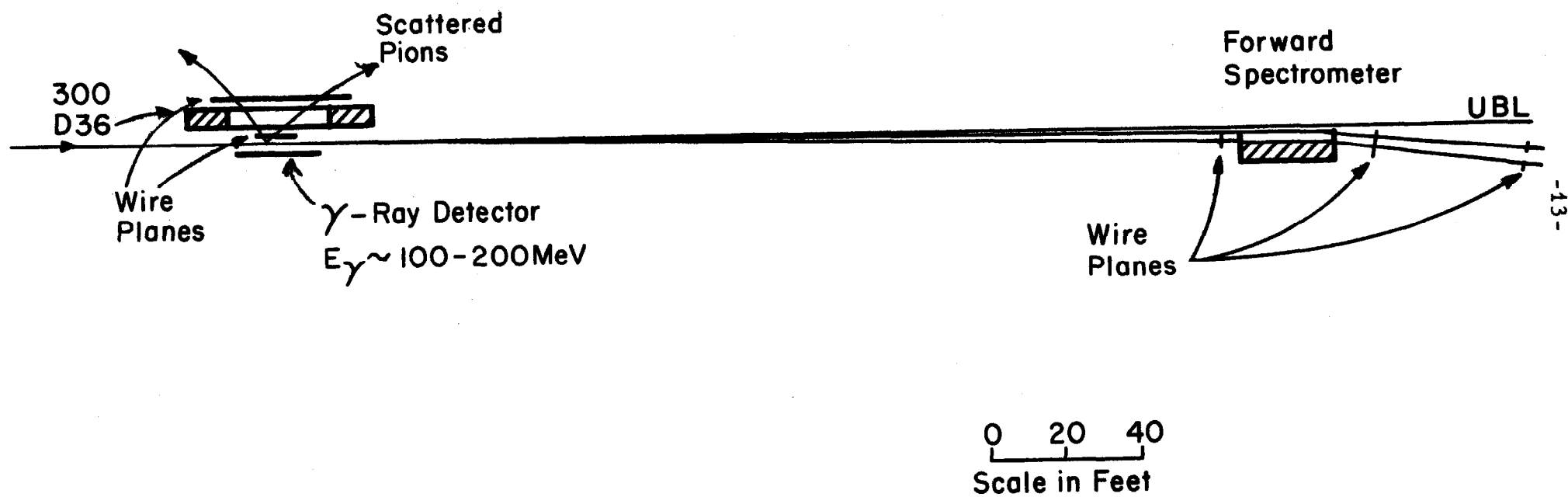
Fig. 3. Layout of experiment showing detectors for both forward and backward particles.
