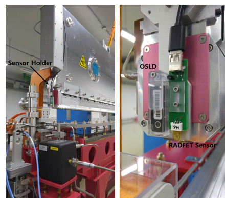
Figure 2: Installation of radFET sensors into undulator. The two sensors were installed into upstream and downstream face of undulator magnet structure [8].
