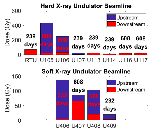
Figure 6: Accumulated radiation dose level of PAL-XFEL undulator segments on July 2019. The undulators with marked 608 days use a Tyndall sensor and other one is REM Oxford Ltd Sensor.
