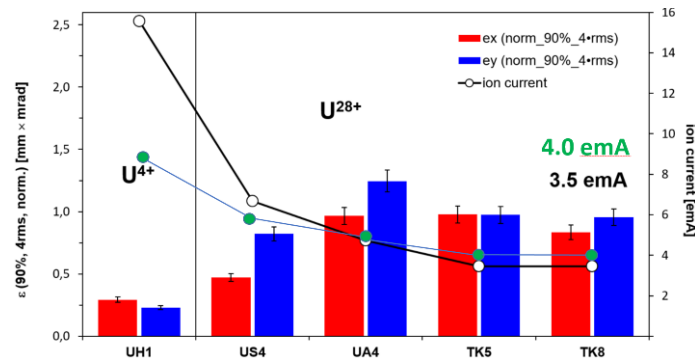
Figure 6. Transversal U^{4+}/28+ emittance along UNILAC [15].
