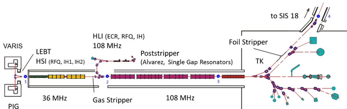
Figure 1. Overview of the GSI Universal Linear Accelerator UNILAC [4].
