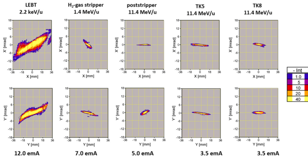
Figure 5. Transversal U^{4+/28+} emittance shape along the UNILAC.
