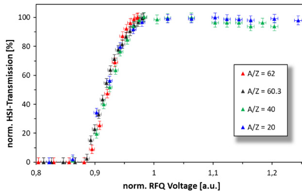
Figure 3. HSI-RFQ working point re-defined [4].
