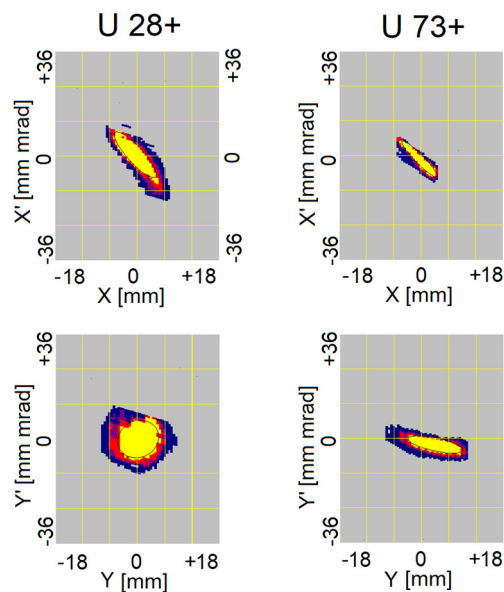
Figure 7. Transversal emittance at TK8, applying pulsed hydrogen gas stripper, 4.0 emA U^{28+} , 1.0 emA U^{73+} (2022).
