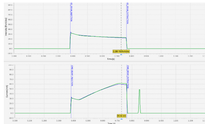
Figure 8. RF capture of the UNILAC beam in the SIS18.
