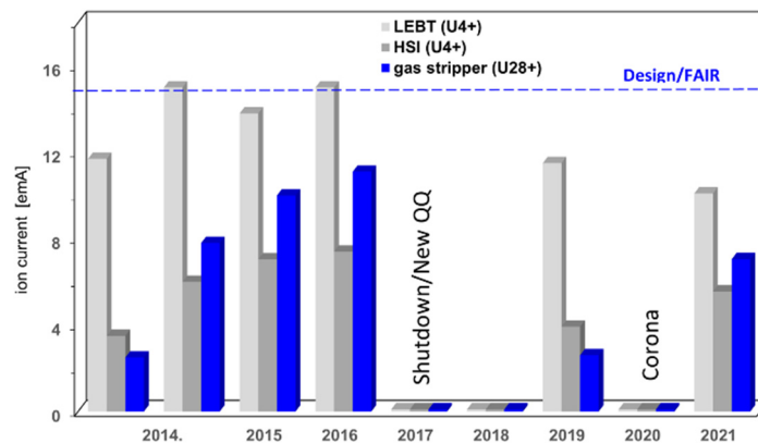
Figure 2. Uranium beam intensity at the UNILAC HSI [4].
