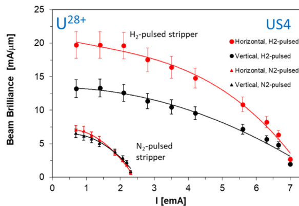
Figure 4. Transversal uranium ( U^{28+} ) beam brilliance behind the gas stripper.
