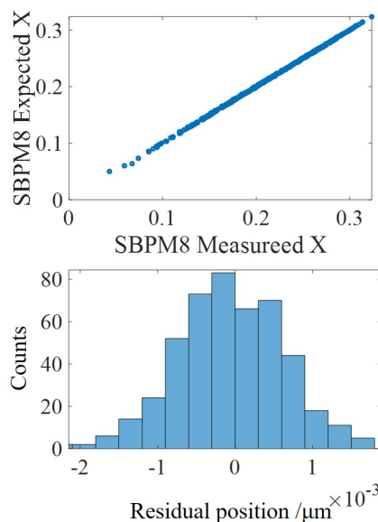
Figure 7: The results of resolution evaluation of the 8th SBPM by neural network.
