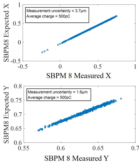
Figure 4: Resolution measurement of the 8th SBPM at SXFEL. (upper) measurement of the horizontal direction; (bottom) measurement of the vertical direction.
