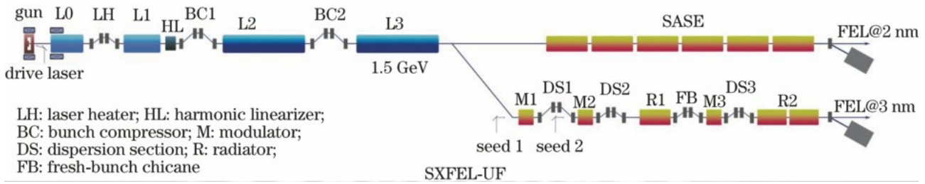
Figure 1: Schematic diagram of SXFEL-UF.
