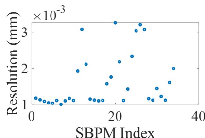
Figure 8: The batch results of resolution evaluation of SBPMs by neural network.
