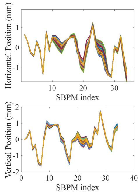
Figure 5: Beam transverse position orbit data in a period of time in SXFEL-UF. (upper) orbit data in the horizontal direction; (bottom) orbit data in the vertical direction.
