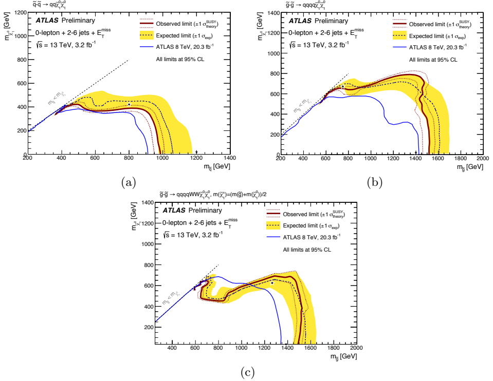
Fig. 2. (Colour on-line) 95% C.L. exclusion limits for direct production of light-flavour squark pairs decaying to one quark and \tilde{\chi}_1^0 with decoupled gluinos (a), gluino pairs decaying to two quarks and \tilde{\chi}_1^0 with decoupled squarks (b) and gluino pairs decaying via an intermediate \tilde{\chi}_1^0 to two quarks, a W boson and a \tilde{\chi}_1^0 for models with a fixed m_{\tilde{\chi}_1^\pm} = (m_{\tilde{g}} + m_{\tilde{\chi}_1^0})/2 (c). The dashed (blue) lines show the expected limits at 95% C.L., with the grey (yellow) bands indicating the 1\sigma excursions due to experimental and background-only theoretical uncertainties. Observed limits are indicated by thick black (maroon) curves where the solid contour represents the nominal limit, and the dotted lines are obtained by varying the signal cross section by the theoretical uncertainties. Results are compared with the observed limits obtained by Run 1 ATLAS search. Taken from Ref. [31].
