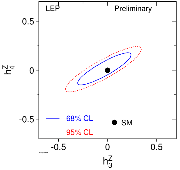
Figure 11.6: Contour curves of 68% C.L. and 95% C.L. in the planes (h_1^\gamma, h_2^\gamma) , (h_3^\gamma, h_4^\gamma) , (h_1^Z, h_2^Z) and (h_3^Z, h_4^Z) showing the LEP combined result.
