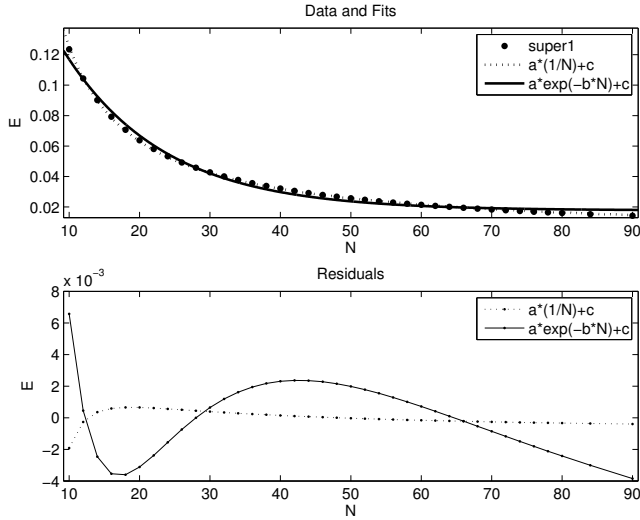
Fig. 9. Ground state energy of supersymmetric extension of bosonic model (11) (depicted as super1 dots) belongs to continuous energy spectrum as manifested by consistency of convergence with 1/(N) fit. The values of R -square = 0.9997 and RMSE = 0.0004644 for 1/(N) fit compared to R -square = 0.9826 and RMSE = 0.002315 for exponential fit favour the linear inverse fit.
