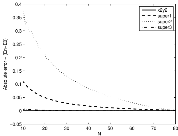
Fig. 7. Comparison of convergence rates of four above mentioned models (bosonic model x^2y^2 , supersymmetric models with both flat directions (super1), with one flat direction (super2) and the toy model with a gap (super3) [12]) reported in previous sections. Absolute error (E_N - E_0) is evaluated considering the reference E_0 calculated at dimension N = 80 , whilst E_N corresponds to energy value at particular dimension N .
