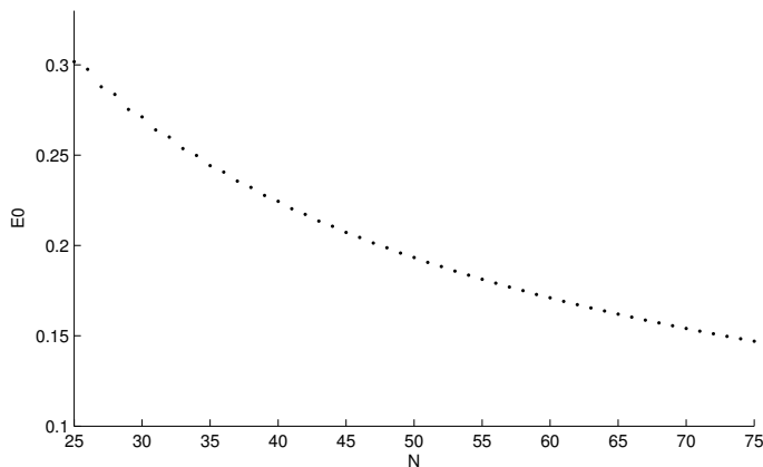
Fig. 5. Convergence of ground state eigenvalue for Hamiltonian with potential with one flat direction (15).
