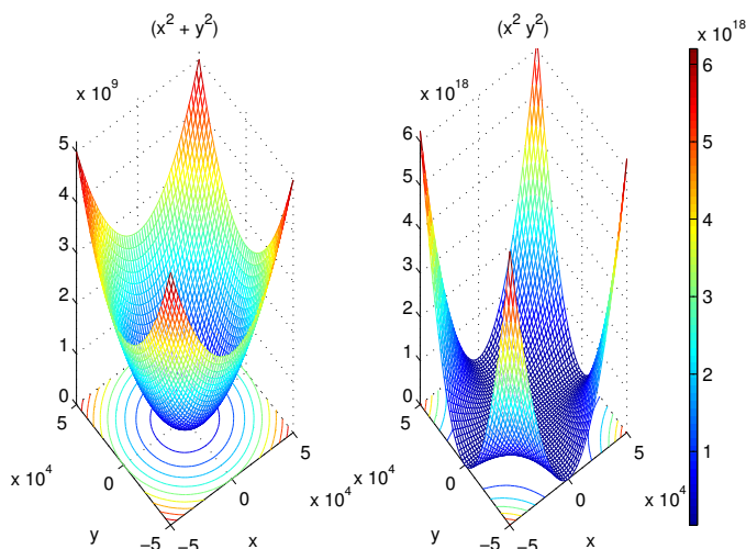
Fig. 1. Comparison of the 2D harmonic potential (left) with x^2 y^2 potential (right).
