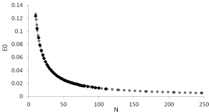
Fig. 3. Depicted convergence of ground state eigenvalue E_0 for the SUSY Hamiltonian (11), calculated for large dimensions of x and p matrices.
