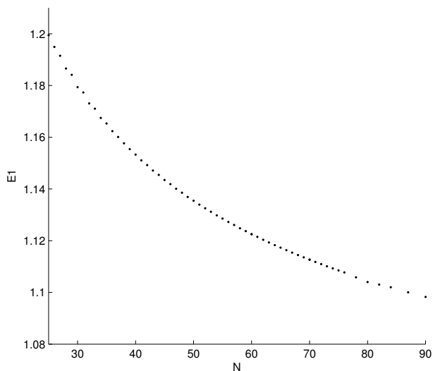
Fig. 4. Convergence of eigenvalue E_1 to value 1 for model Hamiltonian (17) with eigenvalue space spanned by interval [1, \infty] . There is also ground state eigenvalue below E_1 as reported in [12].
