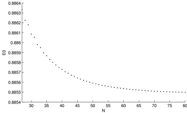
Fig. 6. Convergence of ground state eigenvalue for model Hamiltonian (17) with potential without flat directions [12].
