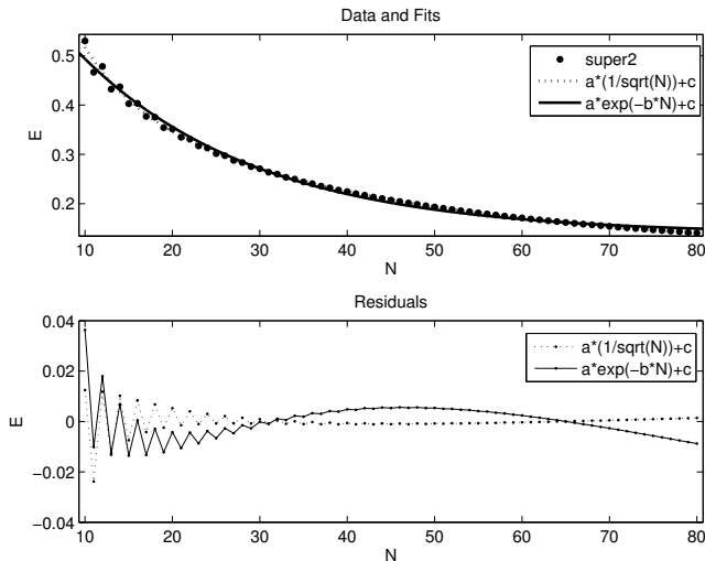
Fig. 10. Model with mass term embedded in one potential valley is characterized by continuous spectrum comprising the interval [0, \infty] . Goodness of fits: Exponential fit — R -square = 0.994; RMSE = 0.007412 ; 1/\sqrt{N} fit — R -square = 0.9977; RMSE = 0.004553 .
