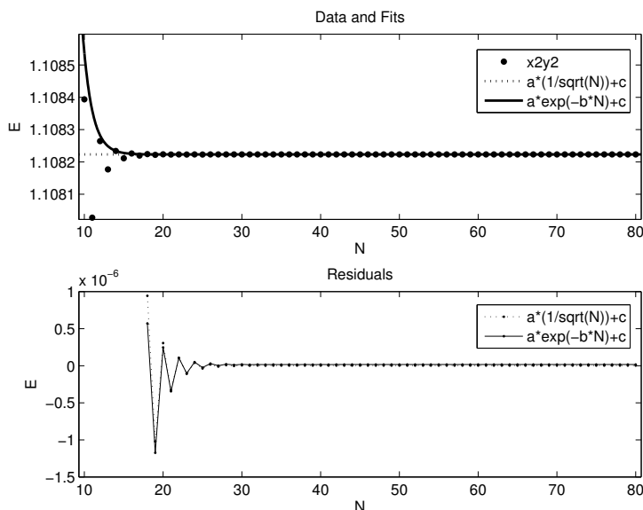
Fig. 8. Tight dependence of bosonic x^2 y^2 model (6) ground state eigenvalue on dimension N of p and x matrices on exponential trend indicates and confirms [8] its discrete energy disposition. The convergence is reached at approx. N = 20 . The 1/\sqrt{N} type fit with parameters a = 3.368E - 6 and c = 1.1082 matches up almost constant function. The first 10 cut-off eigenvalues are excluded from fitting procedure as the values at dimension are the prime matter of concern. The residuals for values of E(N) i.e. the differences E(N) - E(N)_{\text{fit}} are given in the bottom subfigure.
