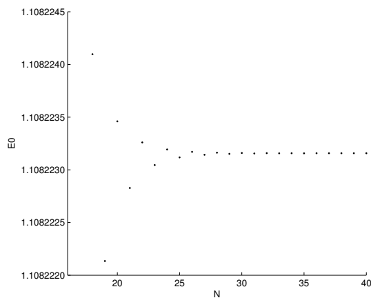
Fig. 2. Convergence of ground state eigenvalue for x^2 y^2 Hamiltonian.
