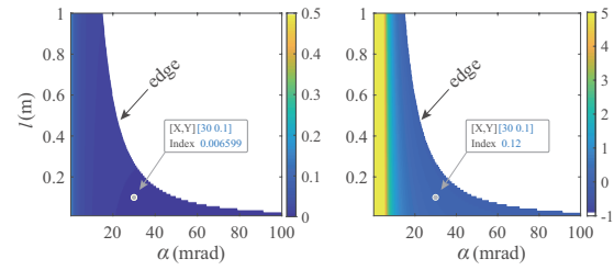
Figure 7: Matched \eta_d (left) and L (right) of dogleg at various bending angle \alpha and length l .
