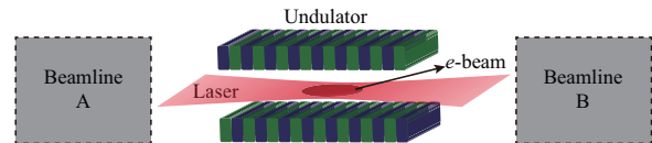
Figure 1: Structure of a compression beamline.
