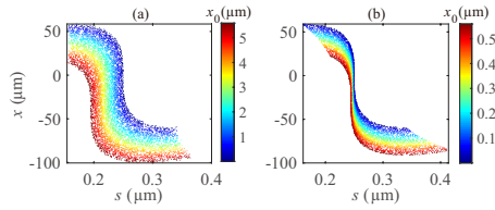
Figure 5: Electron distribution after compression.
