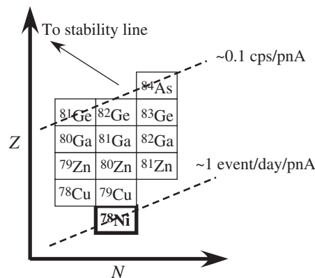
Fig. 6. Nuclear chart related to the ^{78}\text{Ni} mass measurement. The nuclei to be injected into the rare-RI ring accompanied by the ^{78}\text{Ni} beam are shown. Broken lines show the rate in the rare-RI ring. The calculation was done by using LISE++ [25].
