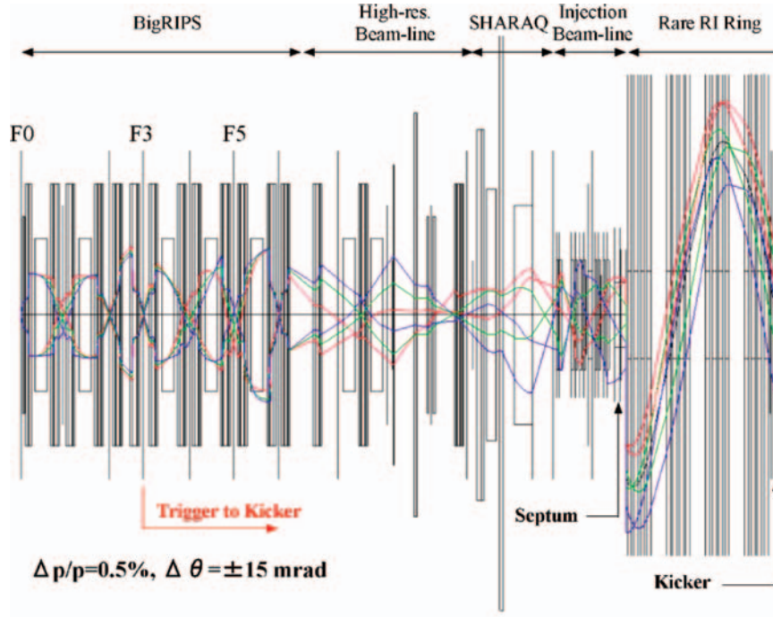
Fig. 5. Ion-optical calculation of the injection beam-line (from F0 in BigRIPS to the kicker magnets in the cyclotron-like storage ring). Red, green, and blue lines correspond to particles with \delta p/p = +0.5\% , 0.0\% , -0.5\% , respectively.
