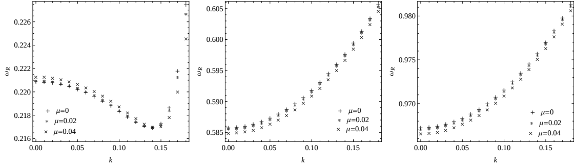
Figure 2. Variety of the real part quasinormal frequencies ( n = 0 ) for the phantom scalar perturbations with k for different \mu . The left, middle and right are for l = 0 , l = 1 and l = 2 .
