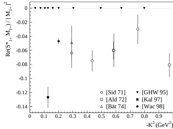
Fig. 4. -K^2 -dependence of the \frac{Re(S_{1+}^* M_{1+})}{|M_{1+}|^2} ratio and the marked -K^2 points of the proposed and completed ELAN experiment [13].
