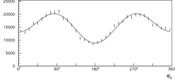
Fig. 3. Fit to the \varphi_\pi -modulation for \vartheta_p^* < 50^\circ .
