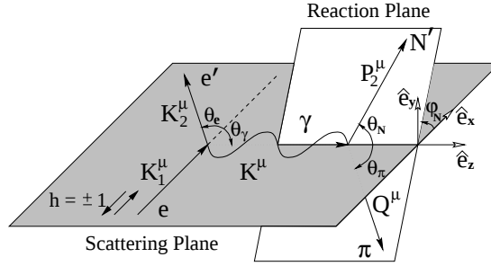
Fig. 1. Kinematics of the \pi -electro-production.
