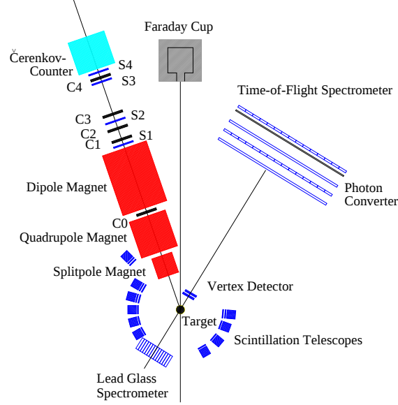
Fig. 2. Schematic experimental set-up.
