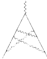
Fig. 2. A corner-ladder vertex graph
