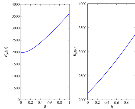
Figure 5. E_N(\rho) for the model (Equation (15)), as a function of h (right-side) for a value of coupling \mu as \mu = 0.9 , and for a value of h = 1.0 held fixed (left-side).
