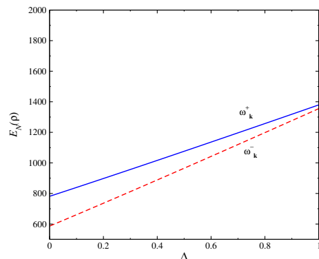
Figure 3. E_N(\rho) as a function of \Delta for H = 1.1 for the model (Equation (1)). We find the negativity entanglement is finite at XY limit ( \Delta = 0 ), increasing with \Delta up to isotropic limit \Delta = 1 .
