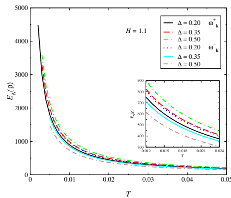
Figure 2. Entanglement negativity E_N(\rho) vs. T for different values of \Delta at H = 1.1 for the model (Equation (1)). We obtain a small negative difference of the entanglement for the bands \omega_{\mathbf{k}}^+ and \omega_{\mathbf{k}}^- (solution of Equation (9)). Furthermore, the entanglement negatively diverges at limit T \rightarrow 0 due to large increases in the quantum fluctuations near T = 0 , where a quantum phase transition takes place.
