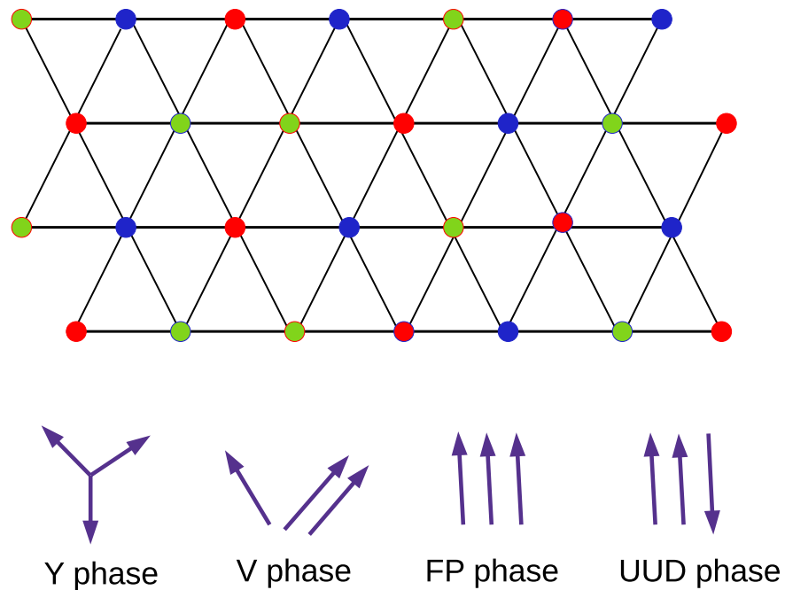
Figure 1. Representation of the triangular lattice for the model from Equation (1), with the three sublattices denoted as A, B , and C . Below, we have the four different spin orientations on A, B , and C sublattices.
