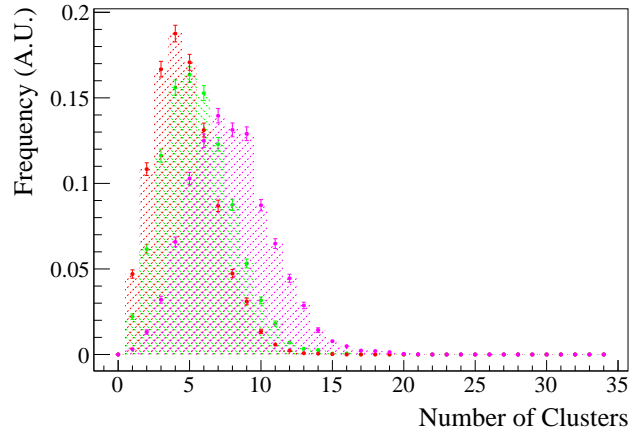
Figure 9.16 The effect of the QE on the photon yield is shown using simulated data. The magenta curve shows the expected number of photons with the QE of the November beam test MCP-PMT. The green and red curves show the expected number of photons where the QE pre and post June beam test has been applied, respectively.
