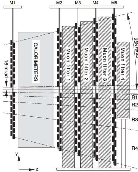
Figure 3.15 Schematic overview of the five muon chambers [25].
