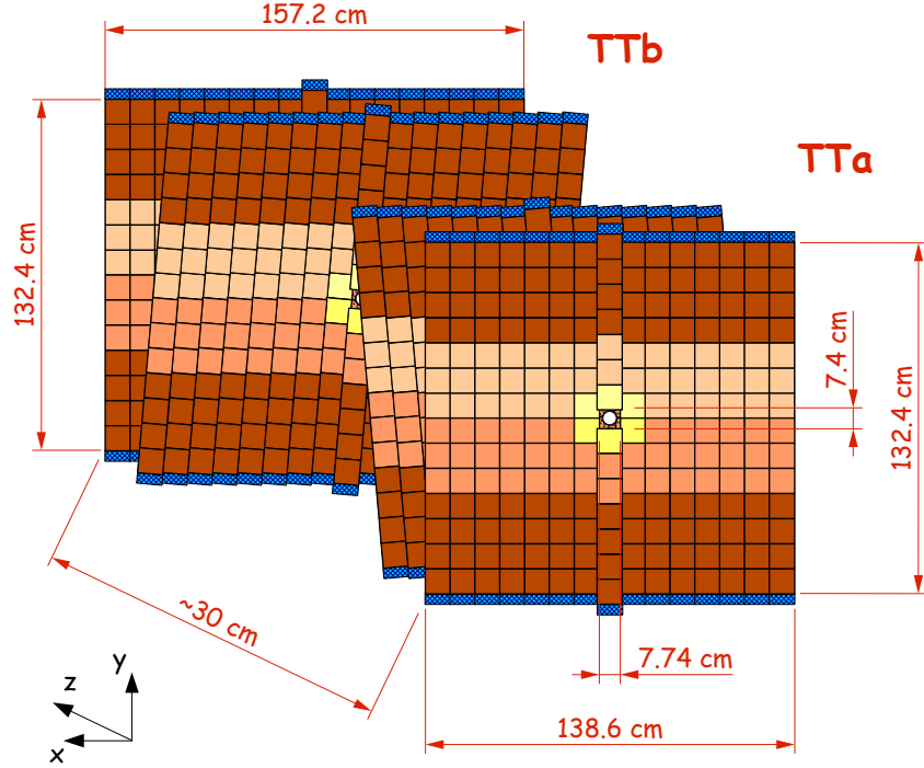
Figure 3.7 Layout and dimensions of the four layers in the Tracker Turicensis, where the sensor placement is indicated by the different shades of brown [25].
