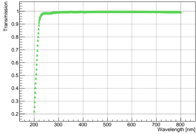
Figure 9.4 The transmission curve of Pactan 8030 adhesive, used to glue the quartz plate and focusing block together. Plot adapted from [80].
