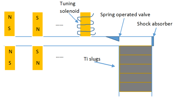
Figure 3: Braking and catching system.
