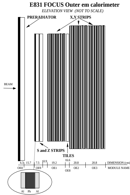
(a) Outer electromagnetic calorimeter layout
