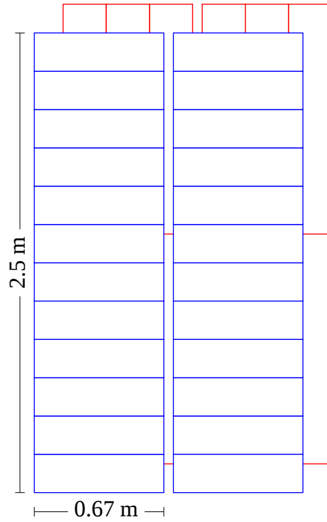
(b) The (H \times V) hodoscope arrays.
