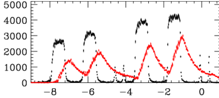
Figure 3.3: Location of primary (black) and secondary (red) for golden mode decays. The primary vertex locations correspond to the position where the target material and the TSSD planes are located. Most of the decay vertices occur outside of this material. Note that the efficiency drops off as the primary vertex is upstream.
