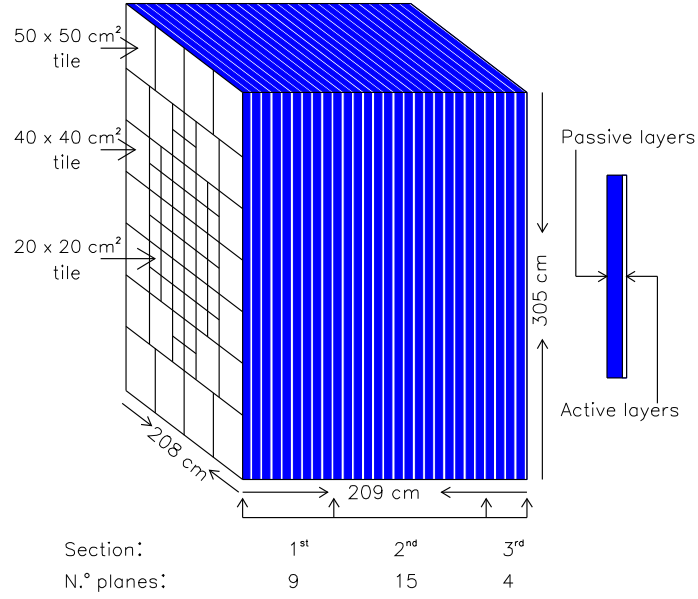
Figure 3.11: Hadron Calorimeter layout.
