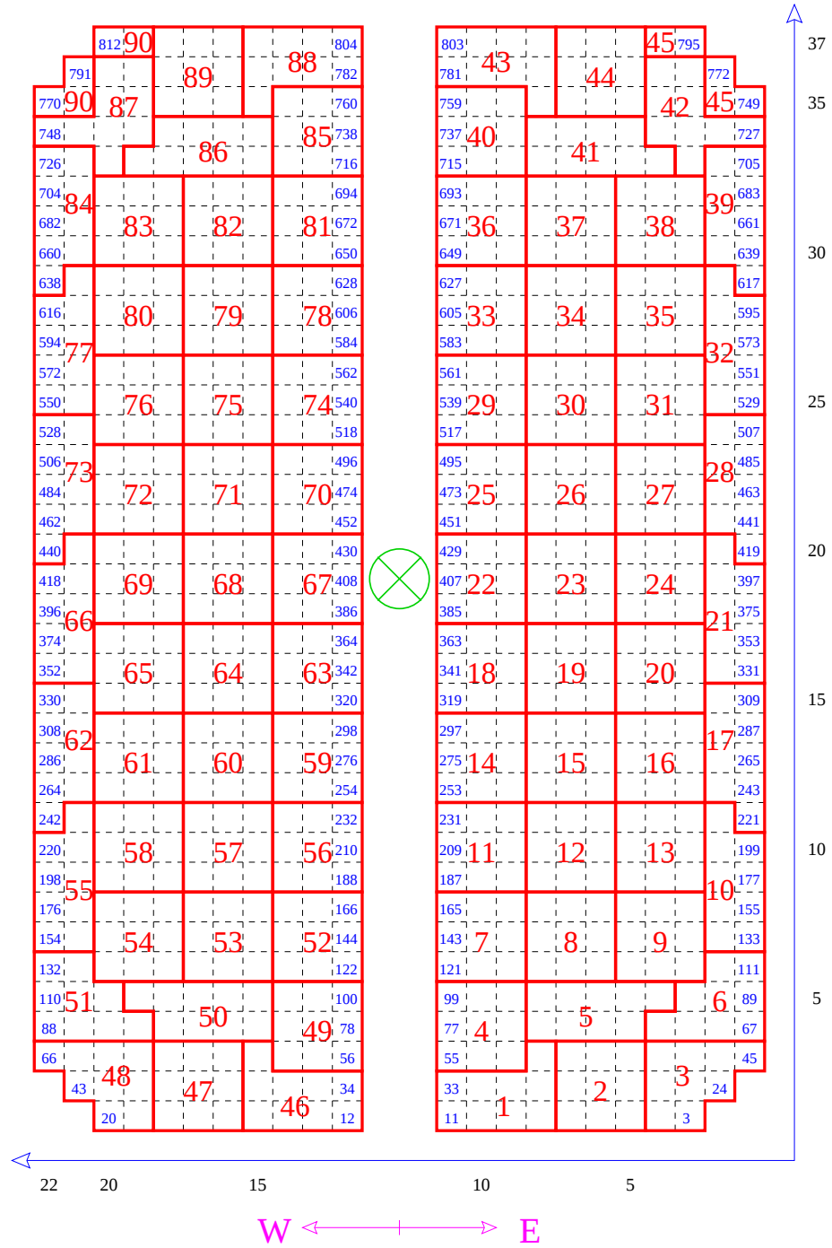
Figure 3.9: Front view of the inner electromagnetic calorimeter.
