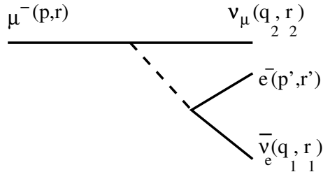
Figure 1.3: The muon decays weakly in an electron a muon neutrino and an electron anti-neutrino.
