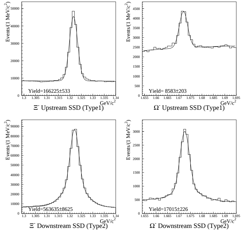
Figure 4.7: The invariant mass plots for the \Lambda\pi^- and the \Lambda K^- combinations for the category where the decays occurs upstream (top row) and downstream (bottom row) of the SSD detector. The plots are for the full FOCUS data sample.
