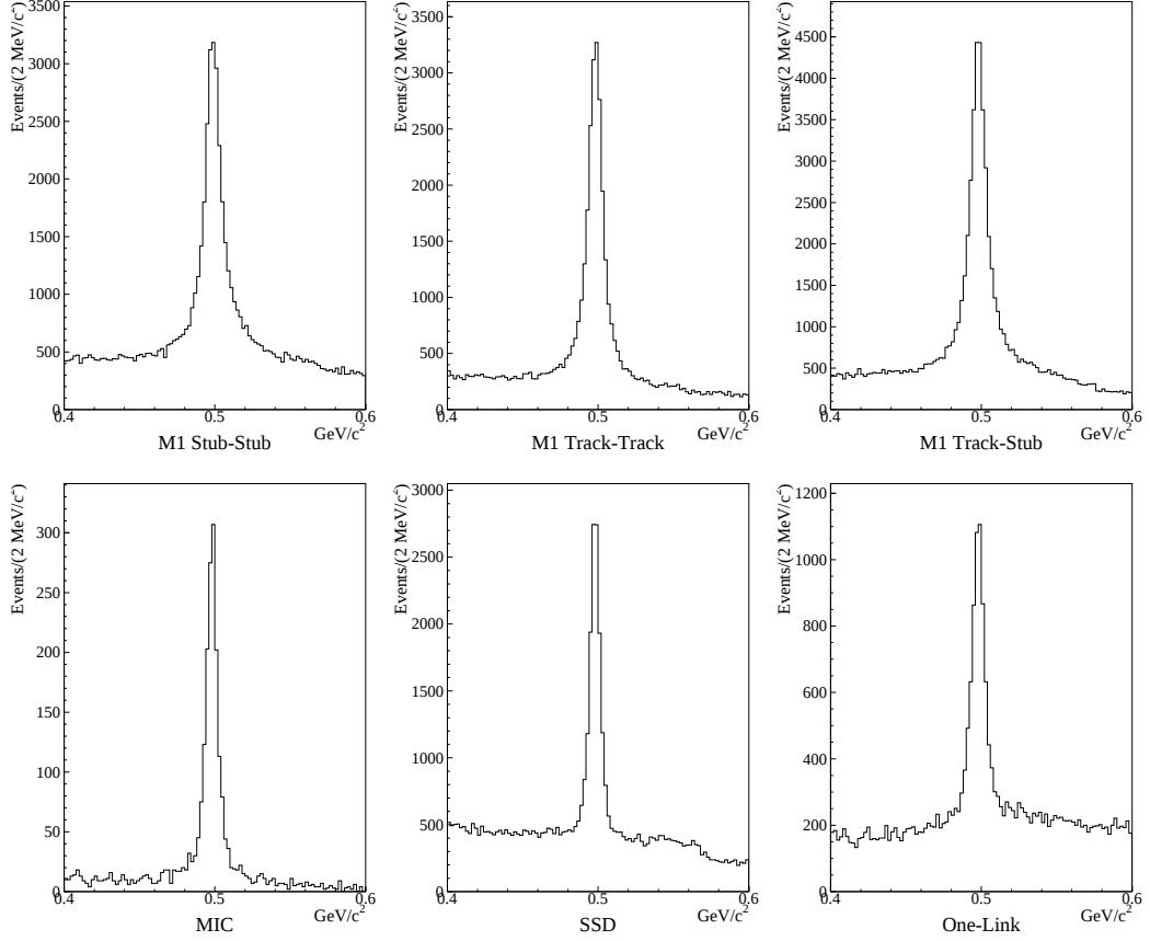
Figure 4.3: Invariant mass distributions for six categories of K_S^0 's. The distributions come from a small sample of runs and include non charm events. The dominant categories in charm decays are the ( M1 track-track ) and ( M1 track-stub ) Vees.
