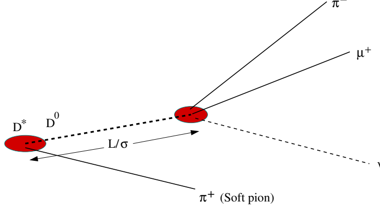
Figure 5.1: Topology of the D^0 semileptonic decays reconstructed in this analysis.
