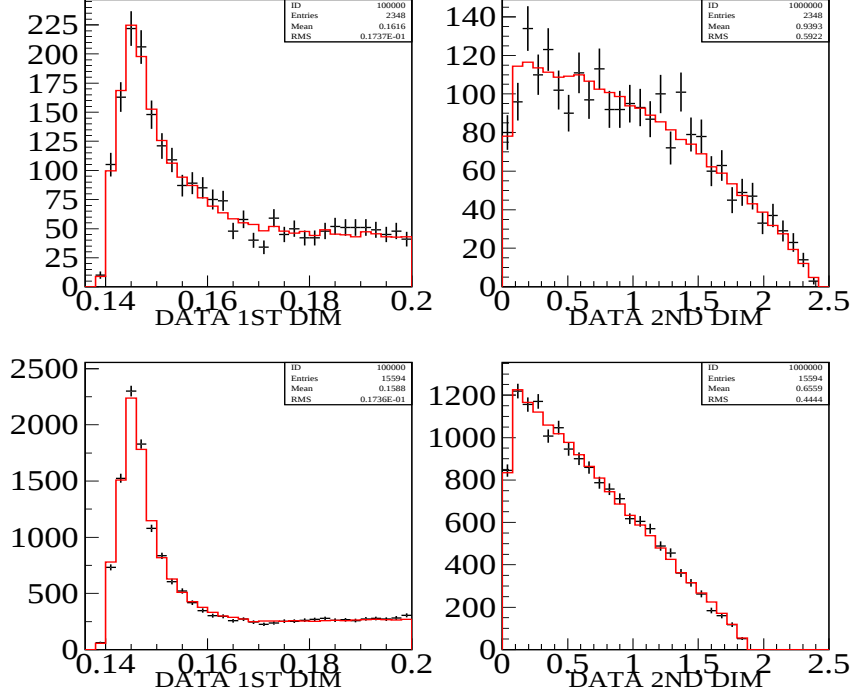
Figure 7.11: Projections of the fit to the D^{*+} - D^0 mass difference vs. q^2 two-dimensional distribution. The top row shows the \pi^- \mu^+ \nu projections while the bottom row shows the K^- \mu^+ \nu projections.
