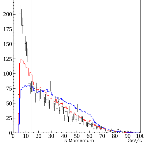
Figure 5.2: The plot shows the cut on the pion momentum. The data (points with error bars) is overlaid with a dedicated Monte Carlo of \pi^- \mu^+ \nu (blue histogram) and with a c\bar{c} Monte Carlo (red histogram). The distributions are normalized by area. We reject events below the the black line.
