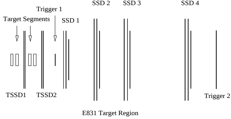
Figure 3.4: Schematic overview of the FOCUS target silicon region.
