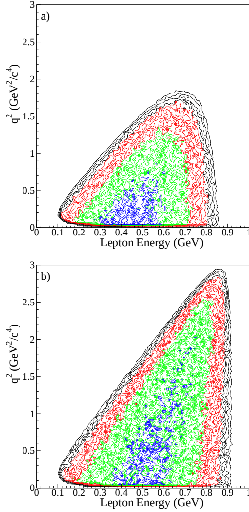
Figure 1.11: Dalitz plot of the decays D^0 \rightarrow K^- \mu^+ \nu (a) and D^0 \rightarrow \pi^- \mu^+ \nu (b) as a function of the variables q^2 and lepton energy. The blue region indicates the highest decay intensity.
