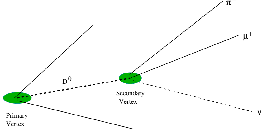
Figure 4.1: Event topology for a semileptonic decay.
