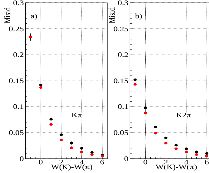
Figure 7.16: Actual misidentification in data (black) and Monte Carlo (red) for: a) D^0 \rightarrow K^- \pi^+ and b) D^0 \rightarrow K^- \pi^+ \pi^+ .
