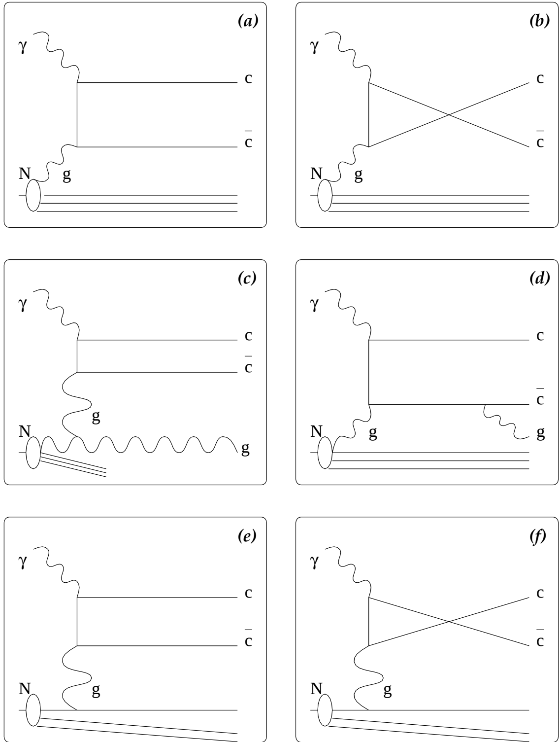
Figure 1.16: Contributions to the photon-gluon fusion process. The photon from the beam interacts with a gluon from the target creating a c\bar{c} pair.
