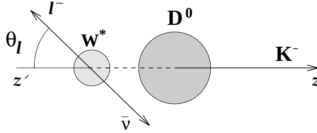
Figure 1.14: The angle \theta_l is defined as the angle between the direction of the charged lepton in the W^* rest frame and the direction of the W^* in the meson M rest frame.
