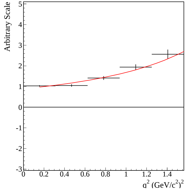
Figure 8.5: Fit to |f_+(q^2)|^2 using a pole mass dependent functional form. The fit returns a pole mass which is in very good agreement with the result obtained from the parametric analysis.
