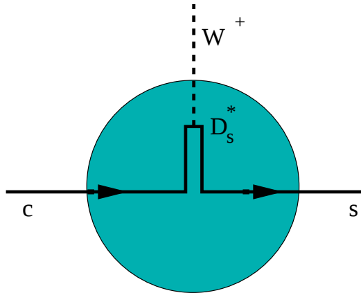
Figure 1.10: Graphical representation of the pole dominant parameterization of the form factor. The W^+ couples to an intermediate state formed by a c and an \bar{s} state with the same quantum numbers as the W^+ . The first state available is the D_s^* (2114).
