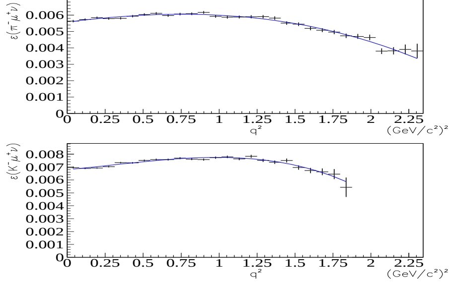
Figure 6.8: Fit to the efficiency as a function of the q^2 for both D^0 \rightarrow \pi^- \mu^+ \nu (top) and D^0 \rightarrow K^- \mu^+ \nu (bottom).
