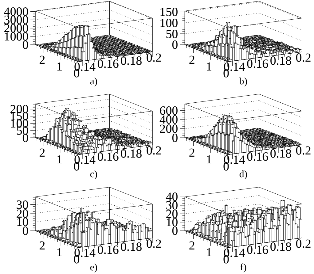
Figure 6.3: D^* - D mass difference versus q^2 . Monte Carlo distributions of the shapes used to fit \pi^- \mu^+ \nu sample. a) \pi^- \mu^+ \nu , b) K^- \mu^+ \nu , c) K^0 \pi^- \mu^+ \nu , d) \rho^- \mu^+ \nu , e) K^- \pi^0 \mu^+ \nu and f) background shape generated using a c\bar{c} Monte Carlo sample where the modes a)-e) have been removed.
