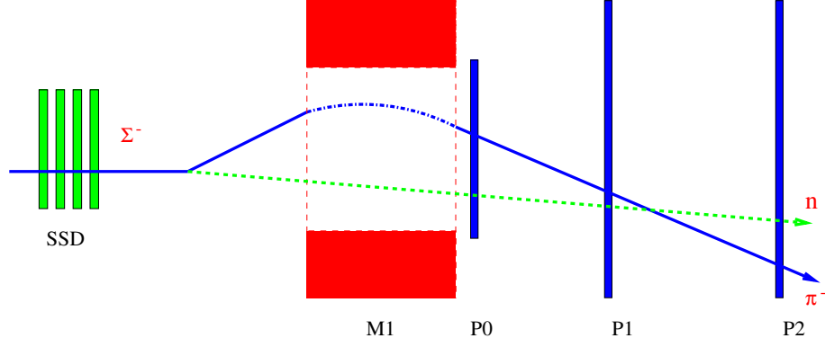
Figure 4.4: Topology of a “kink” in the FOCUS spectrometer.
