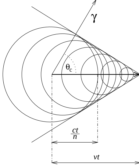
Figure 3.7: The Čerenkov cone depends on the index of refraction of the medium and the speed of the particle.
