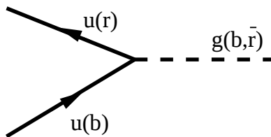
Figure 1.4: Strong vertex where an up-blue quark converts to an up-red quark by emission of a gluon.
