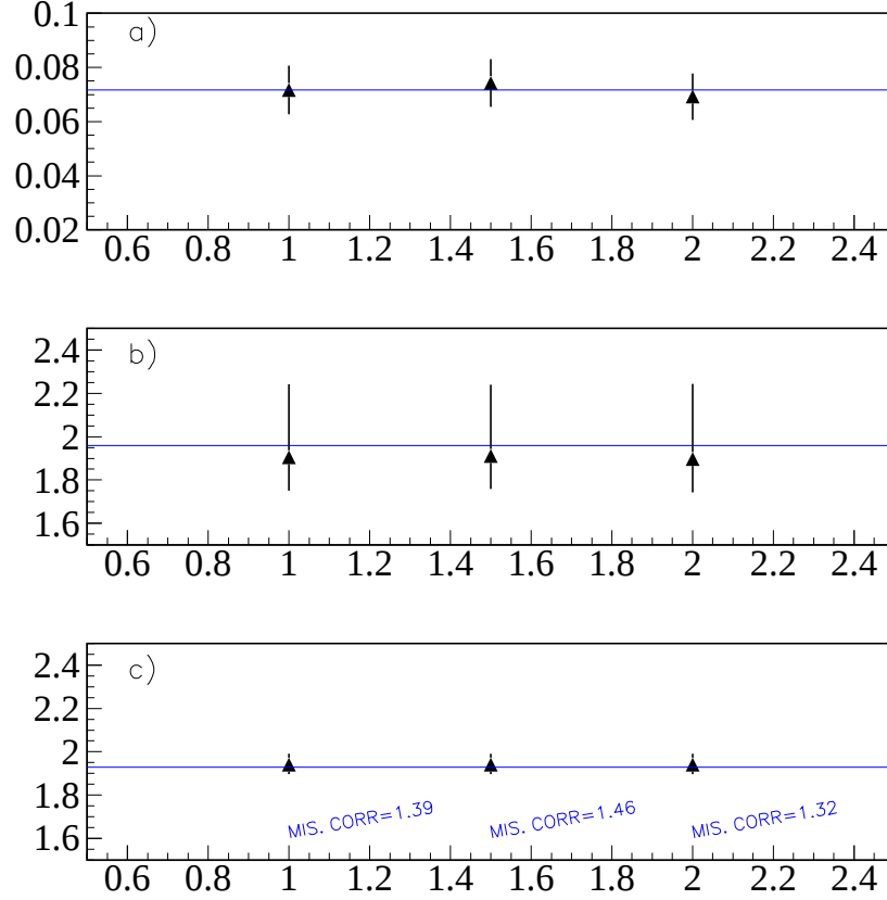
Figure 7.18: a) Relative branching ratio. b) \pi^- \mu^+ \nu pole mass. c) K^- \mu^+ \nu pole mass. We tested the dependence of these parameters from the K \rightarrow \pi misidentification rate. We varied the correction to the Monte Carlo of \pm 1\sigma where \sigma is given by the statistical uncertainty obtained from the study performed on D decays to K^- \pi^+ and K^- \pi^+ \pi^+ . For each tested parameter, the three points correspond to a misidentification rate correction of 1.39, 1.46, and 1.32, respectively.
