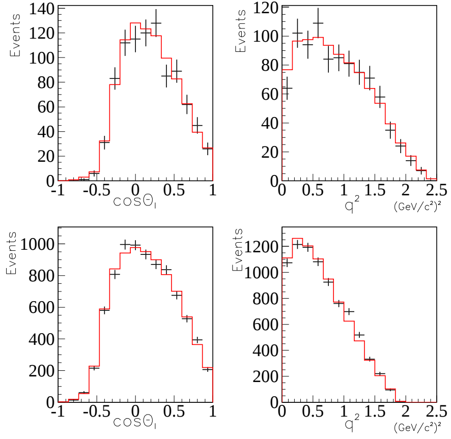
Figure 6.5: Two-dimensional fit projections for K^- \mu^+ \nu and \pi^- \mu^+ \nu .
