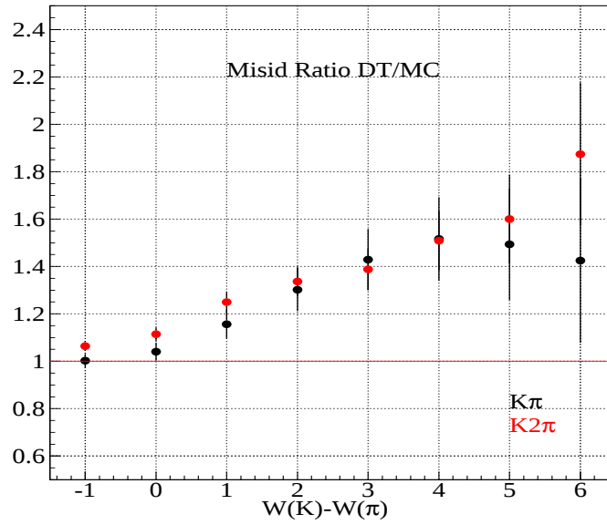
Figure 7.17: The ratio of the misidentification rate between data and Monte Carlo for different piconicity cuts.
