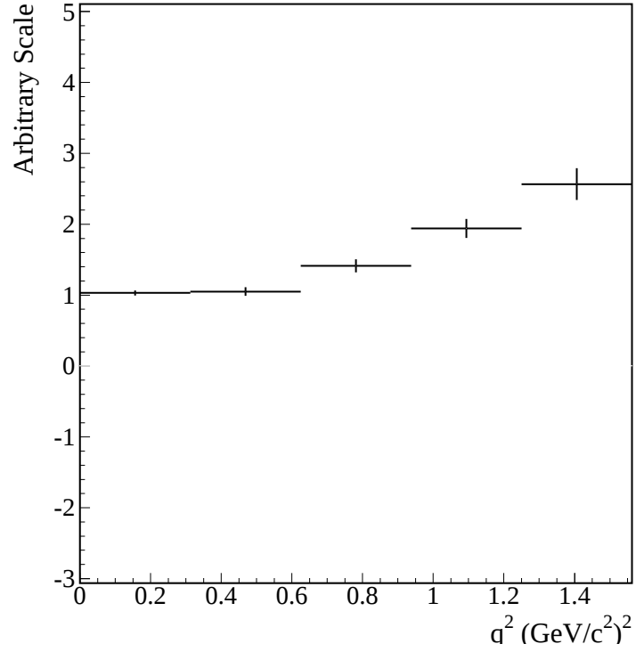
Figure 8.4: D^0 \rightarrow K^- \mu^+ \nu q^2 dependence.
