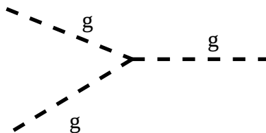
Figure 1.5: Since gluons carry color, strong interaction can couple multiple gluons as well as gluons to quarks.
