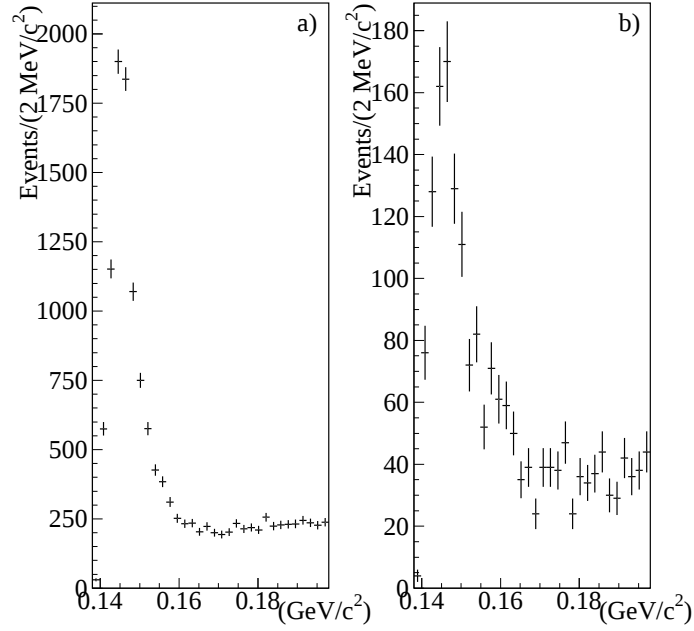
Figure 5.3: D^{*+} - D^0 mass difference distributions after the selection criteria. a) D^0 \rightarrow K^- \mu^+ \nu b) D^0 \rightarrow \pi^- \mu^+ \nu
