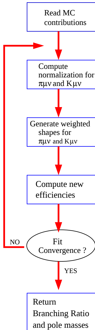
Figure 6.7: Flow diagram describing the steps of the weighting procedure.
