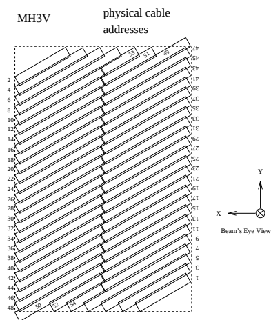
(c) MH3V. MH3U is identical except the counters are rotated by 90^\circ .
