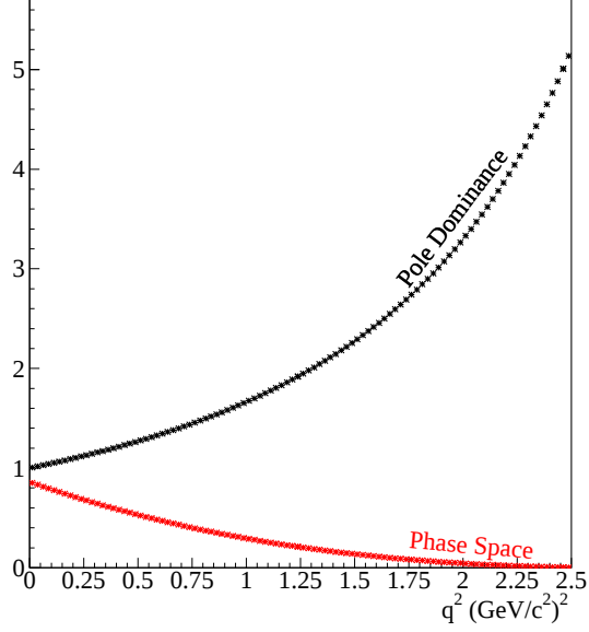
Figure 1.13: Comparison between the pole dominance parametrization of the form factor and the P_K^3 dependence as a function of q^2 .
