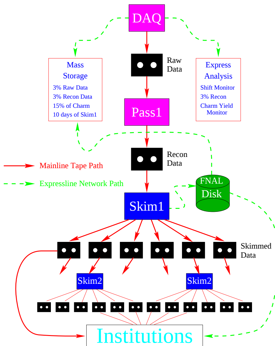
Figure 4.10: Data processing in FOCUS
