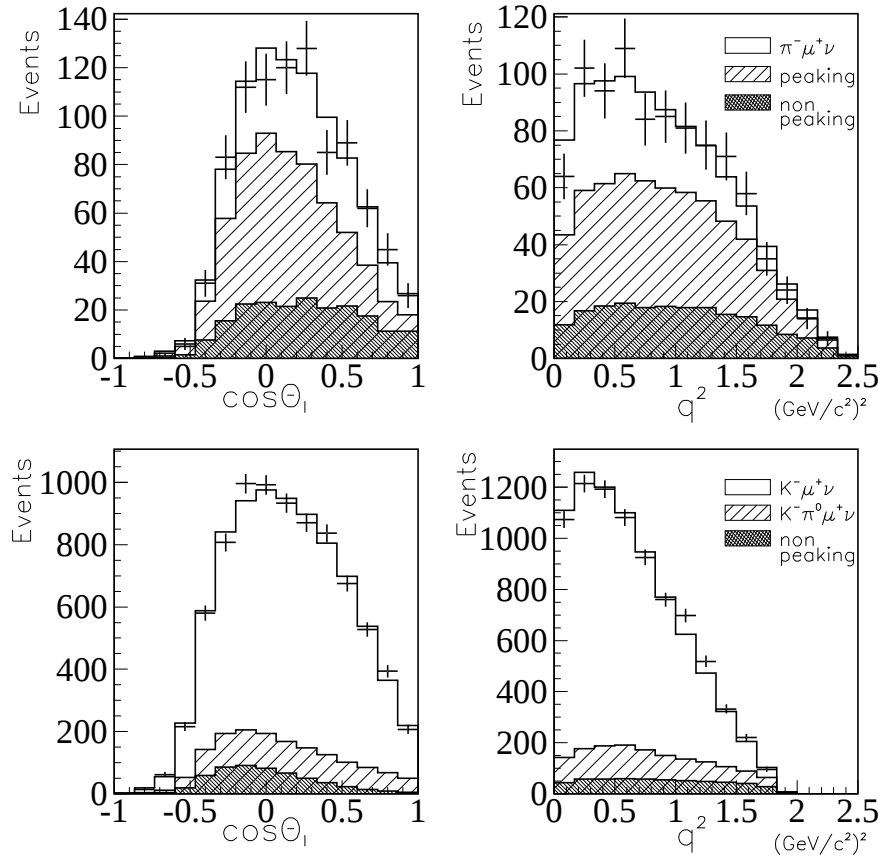
Figure 6.6: Components of the two-dimensional fit for K^- \mu^+ \nu and \pi^- \mu^+ \nu . With the term “non-peaking” we mean the background contribution obtained by a c\bar{c} Monte Carlo with no specific contributions. In the \pi^- \mu^+ \nu plot we refer to the peaking contribution as the sum of \rho^- \mu^+ \nu , K^*(892)^- \mu^+ \nu , and K^- \mu^+ \nu backgrounds.
