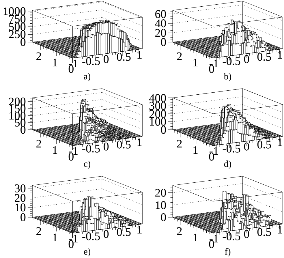
Figure 6.4: \cos\theta_l versus q^2 . Monte Carlo distributions of the shapes used to fit \pi^-\mu^+\nu sample. a) \pi^-\mu^+\nu , b) K^-\mu^+\nu , c) K^0\pi^-\mu^+\nu , d) \rho^-\mu^+\nu , e) K^-\pi^0\mu^+\nu and f) background shape generated using a c\bar{c} Monte Carlo sample where the modes a)-e) have been removed.
