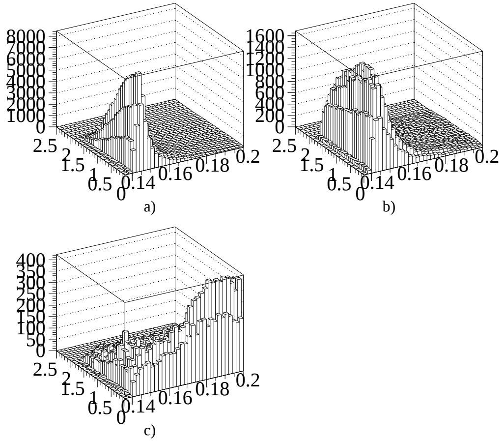
Figure 6.1: D^* - D mass difference versus q^2 . Monte Carlo distributions of the shapes used to fit K^- \mu^+ \nu sample. a) K^- \mu^+ \nu , b) K^- \pi^0 \mu^+ \nu and c) background from a c\bar{c} Monte Carlo sample where the modes K^- \mu^+ \nu and K^- \pi^0 \mu^+ \nu have been removed.
