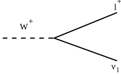
Figure 1.2: Weak process to first order in the S matrix expansion.
