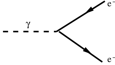
Figure 1.1: Electromagnetic process to first order in the S matrix expansion.
