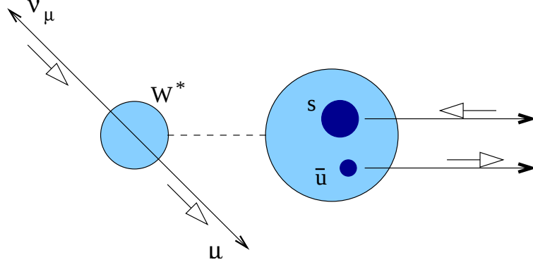
Figure 1.15: The helicity is determined by whether the s quark combine with a quark that has helicity \lambda = +1/2 or \lambda = -1/2 .
