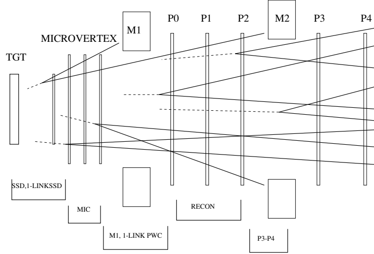
Figure 4.2: Different categories of vees reconstructed in FOCUS .
