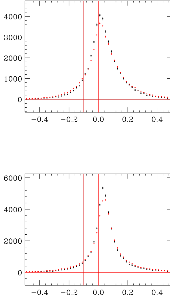
Figure 8.1: Blanking studies using D^0 \rightarrow K^- \pi^+ \pi^+ \pi^+ . In the top plot a comparison of the q^2 resolution between data (black) and Monte Carlo (red) is shown for the standard neutrino closure. At the bottom the same comparison when we apply the D^{*+} cone closure technique. This study has been performed using the decay D^0 \rightarrow K^- \pi^+ \pi^+ \pi^+ .
