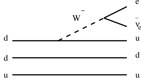
Figure 1.8: In the \beta decay a neutron decays to a proton and a W^- boson and the W decays subsequently to an electron-neutrino pair.
