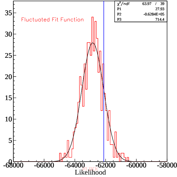
Figure 7.10: The red distribution is obtained by fluctuating the fit function obtained by the fit on the mass difference and q^2 . The fit is obtained using a Gaussian: the parameters p1, p2, and p3 represent the amplitude, the mean and the \sigma of the Gaussian, respectively. The blue line, which indicates the likelihood value returned by the fit to the data is fully compatible with the red distribution.
