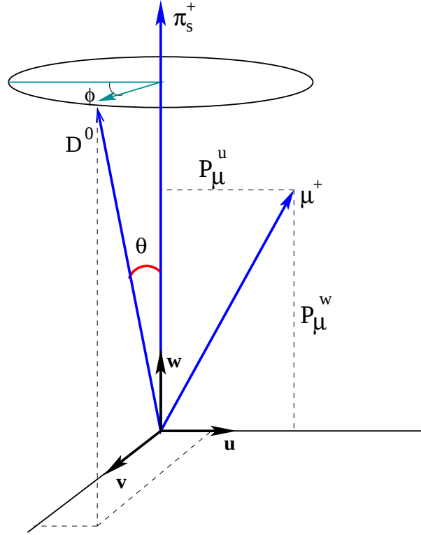
Figure B.1: u\hat{w} frame used in the D^{*+} cone closure
