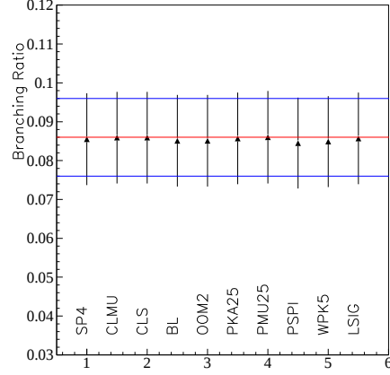
Figure 7.3: \rho^- \mu^+ \nu to K^*(892)^- \mu^+ \nu branching ratio. The blue and red lines show the input value in the weak constraint with relative error. The fit always returns a branching ratio which is consistent with the input value.
