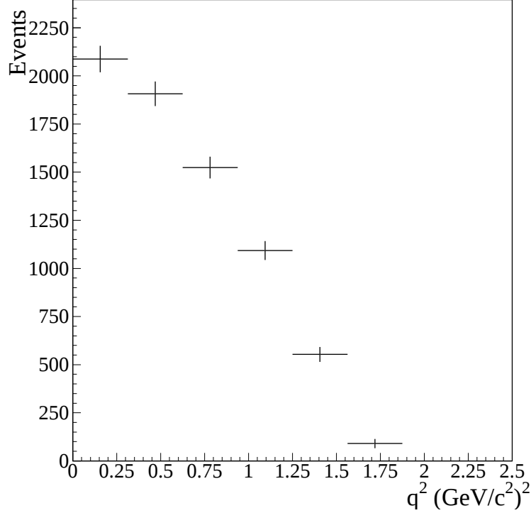
Figure 8.3: Background subtracted q^2 distribution for D^0 \rightarrow K^- \mu^+ \nu . The distribution is obtained by performing a fit to the two dimensional distribution q^2 vs. D^{*+} - D^0 mass difference and subtracting the background components from the total sample.
