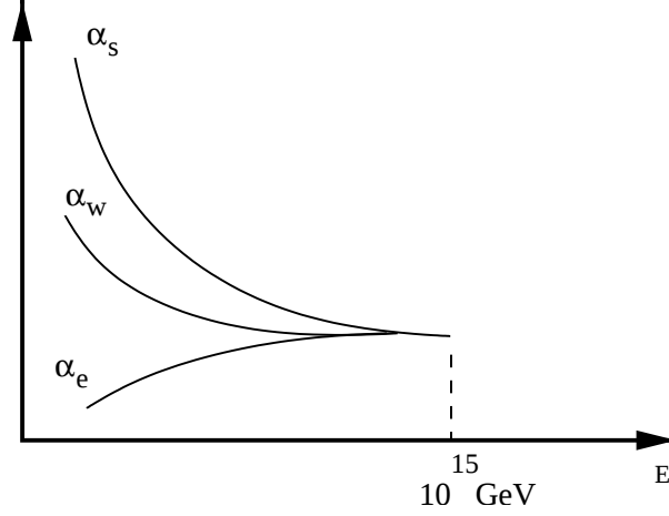
Figure 1.6: The graph shows running coupling constants which (by extrapolation) should converge around 10^{15} GeV.
