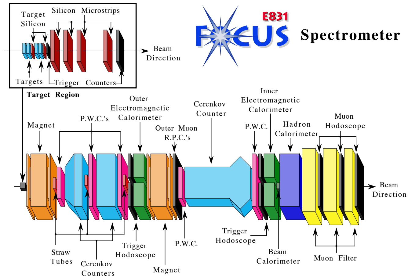
Figure 3.1: Layout of the FOCUS spectrometer.
