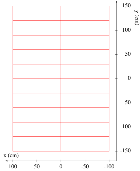
(b) The IM2H array.
