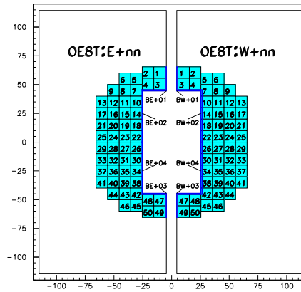
(b) Outer electromagnetic calorimeter layout
