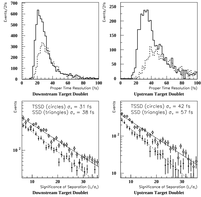
Figure 3.5: Proper time resolution for the decay D^0 \rightarrow K^- \pi^+ . The data is split into events from the most downstream (left column) and the most upstream (right column) pair of BeO segments. Top plots: comparison in the proper time resolution when the target silicon information is included (solid line) and when this information is not included (dashed line). Using the target silicon the fraction of events with good resolution increases. Bottom plots: we show the fit to the number of events as a function of L/\sigma_L . The TSSD improves the proper time resolution significantly.
