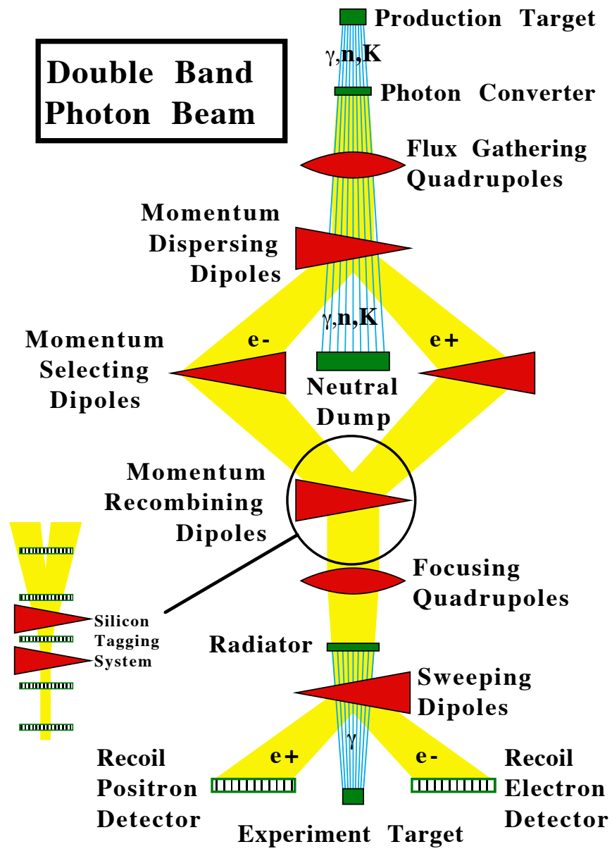
Figure 2.2: Schematic overview of the FOCUS beam line.
