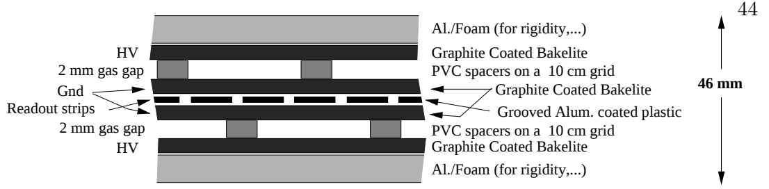
Figure 3.13: RPC modules cross section.
