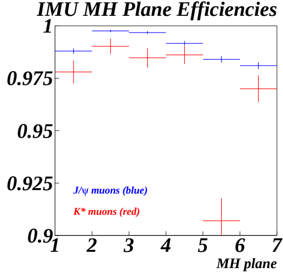
Figure 4.9: MH plane efficiencies computed using J/\psi \rightarrow \mu^+\mu^- and D^+ \rightarrow K^{*}(892)^0\mu^+\nu decays.
