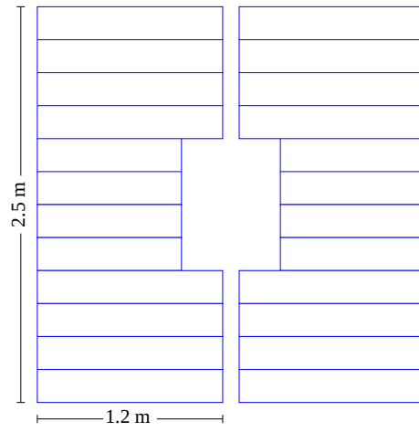
(a) The OH hodoscope arrays.
