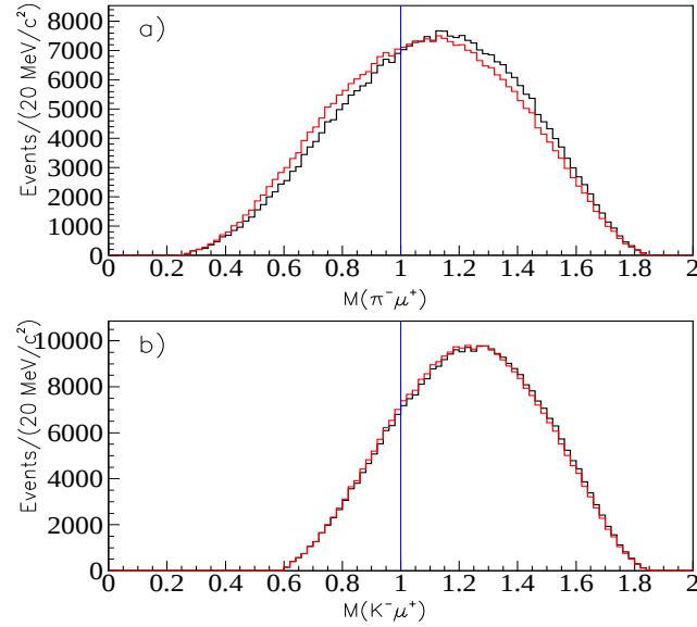
Figure 7.5: Visible mass distributions for different pole masses. a) \pi^- \mu^+ invariant mass distribution for a pole mass equal to 2.10 \text{ GeV}/c^2 (black) and 1.90 \text{ GeV}/c^2 (red). b) K^- \mu^+ invariant mass distribution for a pole mass equal to 2.10 \text{ GeV}/c^2 (black) and 1.90 \text{ GeV}/c^2 (red). The decay D^0 \rightarrow \pi^- \mu^+ \nu is more sensitive to the choice of the pole mass due to the large q^2 reach that better probes the “real pole”.
