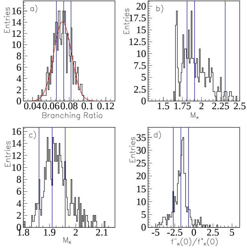
Figure 7.9: These distributions are obtained by fluctuating 500 times the data distributions and fitting each “new” data set following the procedure described in chapter 6. The blue lines show the measured value with relative error ( \pm 1\sigma ) in the fit to the unfluctuated data. a) Branching ratio results: the red curve is the fit of the distribution to a Gaussian shape. b) \pi^-\mu^+\nu pole mass: the plot shows a small pile up of events at the low end tail of the distribution. This effect is an artifact of the fit and is due to the large statistical error on the \pi^-\mu^+\nu pole mass. It reflects the singularity of the pole dominance parametrization of the form factor. c) K^-\mu^+\nu pole mass, d) form factor ratio f_K^-(0)/f_K^+(0) .
