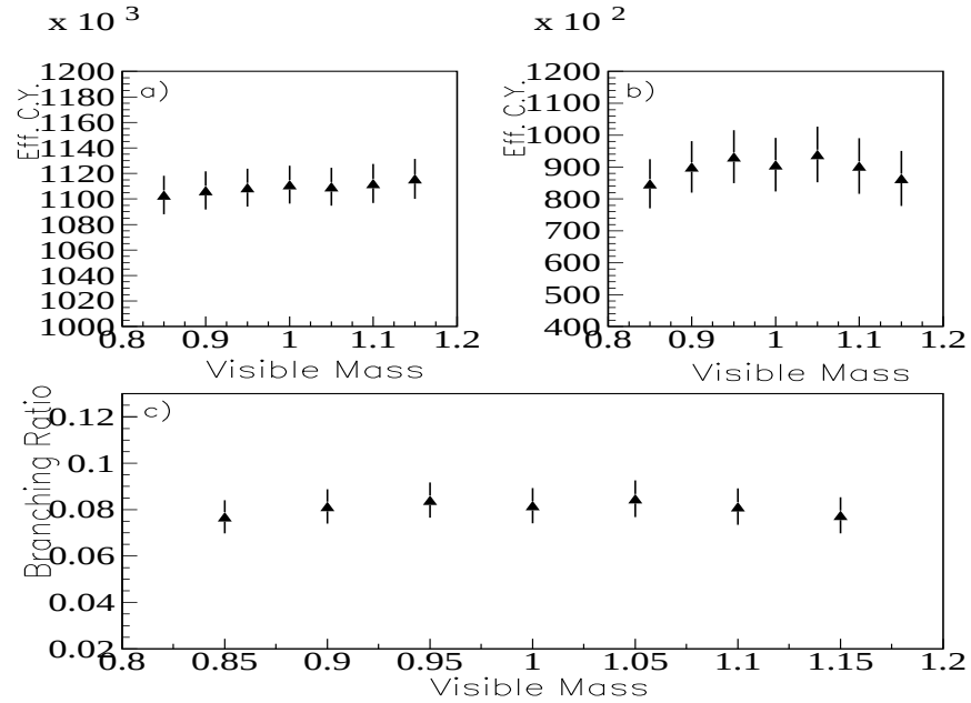
Figure 7.6: Branching ratio for different visible mass cuts.
