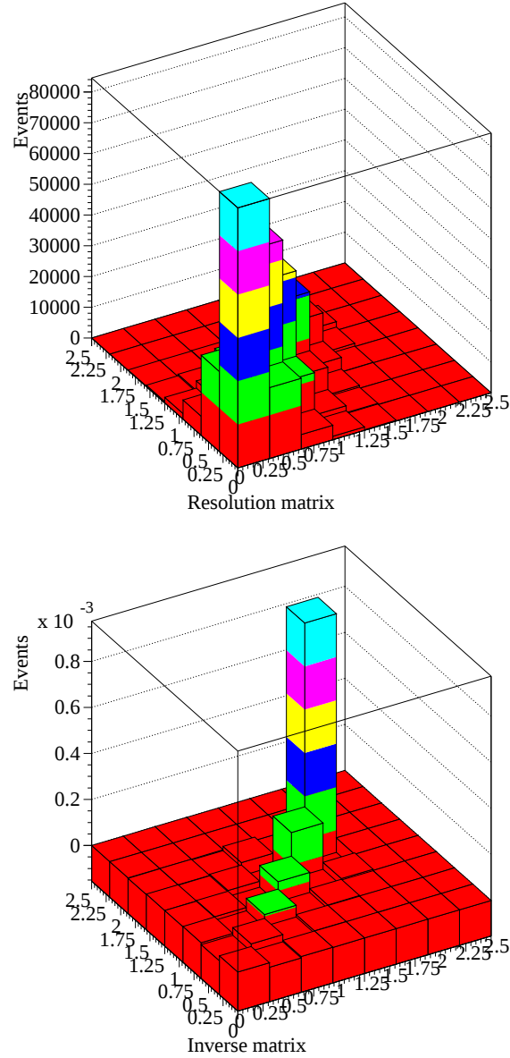
Figure 8.2: (top) Resolution matrix: the non-diagonal terms show the importance of resolution effects in the analysis. We need to account for the fact that in many cases the event is reconstructed in a q^2 bin different from the one where it was generated; (bottom) deconvolution matrix obtained by inversion of the resolution matrix.
