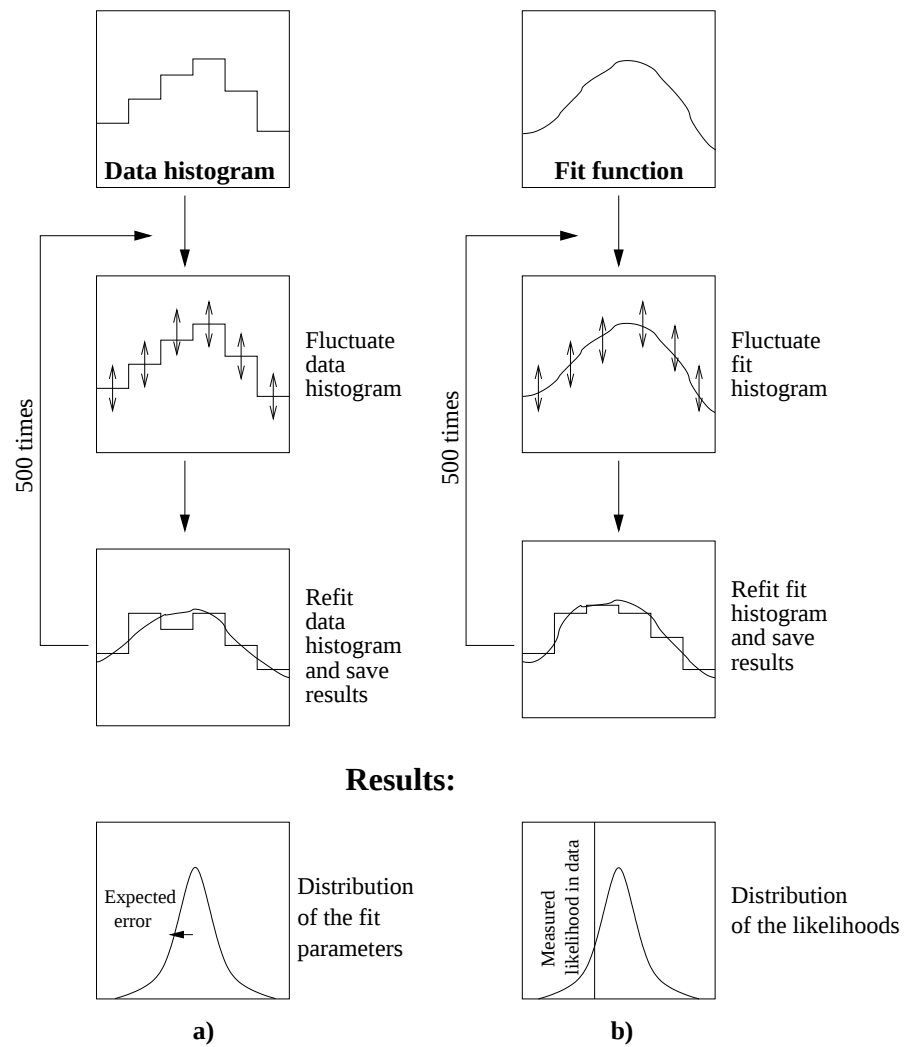
Figure 7.8: The diagrams show the test made to assess the accuracy of the statistical error (a) and of the goodness of fit (b).
