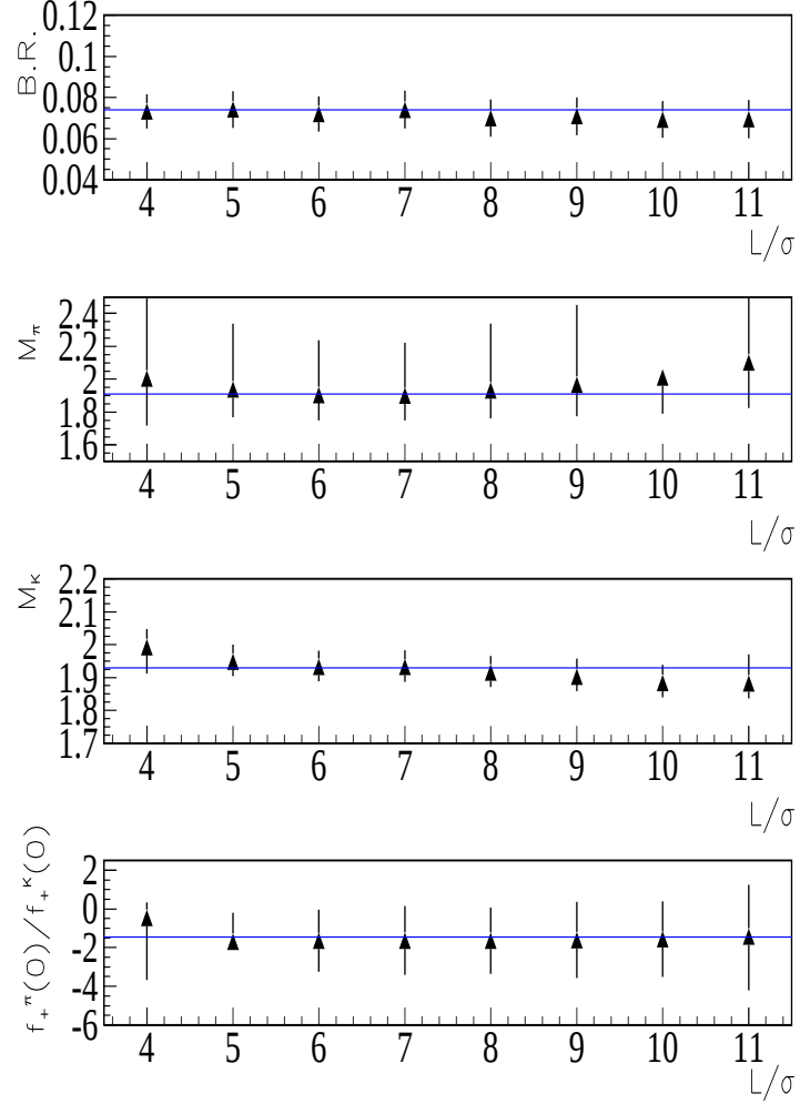
Figure 7.12: Fit results using a fit to the D^{*+} - D^0 mass difference and q^2 fit. The results are in good agreement with the results obtained in the standard fit (blue line).
