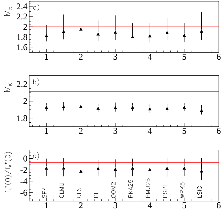
Figure 7.4: Cut variations. The nominal value for these parameters is given by the red line. a) Pole mass for \pi^- \mu^+ \nu . b) Pole mass for K^- \mu^+ \nu . c) Ratio f_K^-(0)/f_K^+(0) for K^- \mu^+ \nu . In all cases the results are consistent with each other. In particular the K^- \mu^+ \nu pole mass is statistically inconsistent with the nominal pole at 2.114 \text{ GeV}/c^2 . Notice that the fit corresponding to the variation PMU25 (muon momentum greater than 25 \text{ GeV}/c ) failed to find the asymmetric errors.
