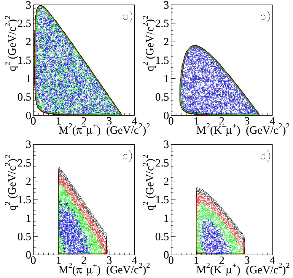
Figure 6.9: a), b) Phase-space before rejection. c), d) Dalitz after rejection on the intensity I' . The left and right columns refer to \pi^- \mu^+ \nu and K^- \mu^+ \nu respectively.
