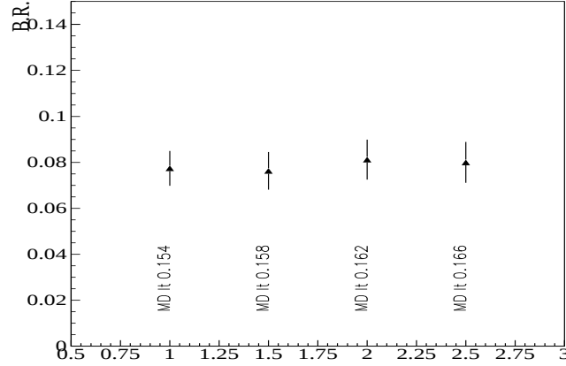
Figure 7.7: \Gamma(\pi^-\mu^+\nu)/\Gamma(K^-\mu^+\nu) branching ratio for different D^{*+}-D^0 mass difference cuts.
