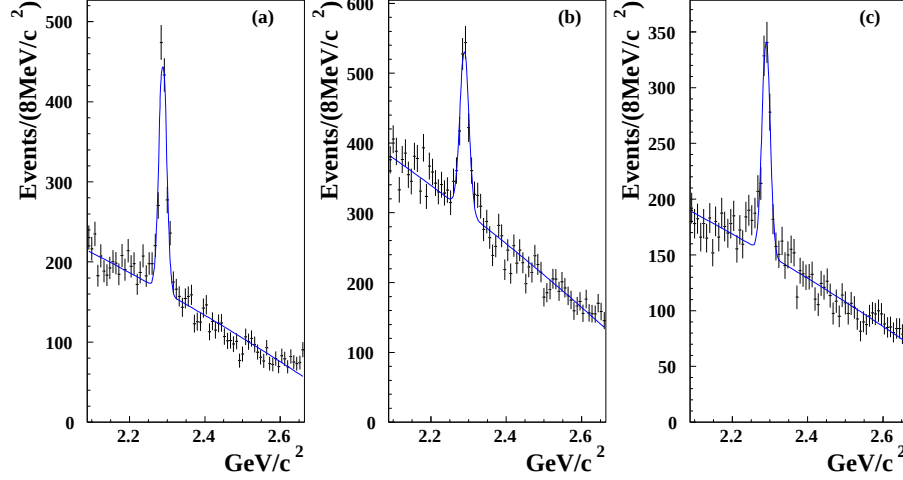
Figure 4.5: Three invariant mass plots for the decays (a) \Lambda_c^+ \rightarrow \Sigma^+ \pi^+ \pi^- where \Sigma^+ \rightarrow p \pi^0 with a yield of 915 \pm 50 events, (b) \Lambda_c^+ \rightarrow \Sigma^+ \pi^+ \pi^- where \Sigma^+ \rightarrow n \pi^+ with a yield of 854 \pm 65 events, and for (c) \Lambda_c^+ \rightarrow \Sigma^- \pi^+ \pi^- where \Sigma^- \rightarrow n \pi^- with a yield of 654 \pm 42 events.
