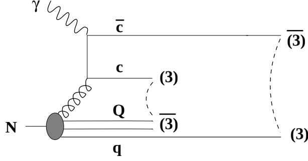
Figure 1.17: In associated charm production the charm quark dresses with the di-quark while the anti-charm quark binds to the remaining quark creating an asymmetry in the particle-antiparticle momentum spectra as well as in the number of meson (baryon) particles and meson (baryon) anti-particles.
