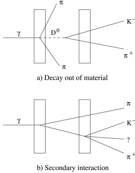
Figure 3.2: a) Decay of a D^0 particle to the final state K^-\pi^+ . The decay occurs out of the target material. b) Example of background from re-interaction of particles coming from the the interaction vertex.
