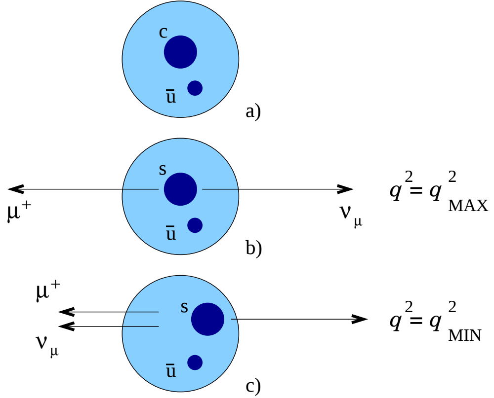
Figure 1.12: Possible kinematic configurations during the hadronization process of a D^0 meson decaying to a kaon: (a) The D^0 meson before the decay; (b) decay configuration for q^2 = q^2_{\text{max}} , where the form factors are large for producing a kaon (or a K^* ) meson in the final state; (c) configuration for q^2 = q^2_{\text{min}} where the form factors are smallest.
