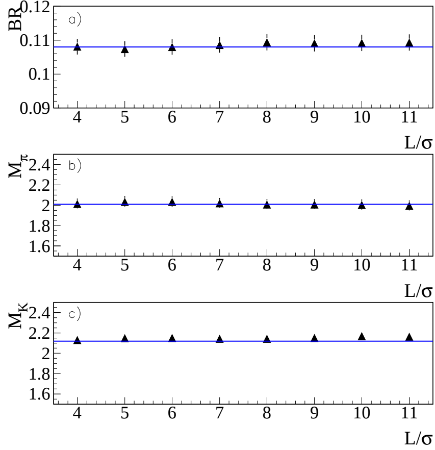
Figure 7.1: Fit to the c\bar{c} Monte Carlo sample for eight different L/\sigma values. The blue line represent the input value in the FOCUS Monte Carlo. a) Relative branching ratio of \pi^-\mu^+\nu to K^-\mu^+\nu . b) \pi^-\mu^+\nu pole mass. c) K^-\mu^+\nu pole mass.
