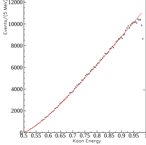
Figure 1.9: Mass term effect on the kaon energy distribution of the decay D^0 \rightarrow K^- \mu^+ \nu : the fit is performed using a functional form that neglects the mass term and it shows that this approximation works very well up to the high edge of the kaon energy spectrum.
