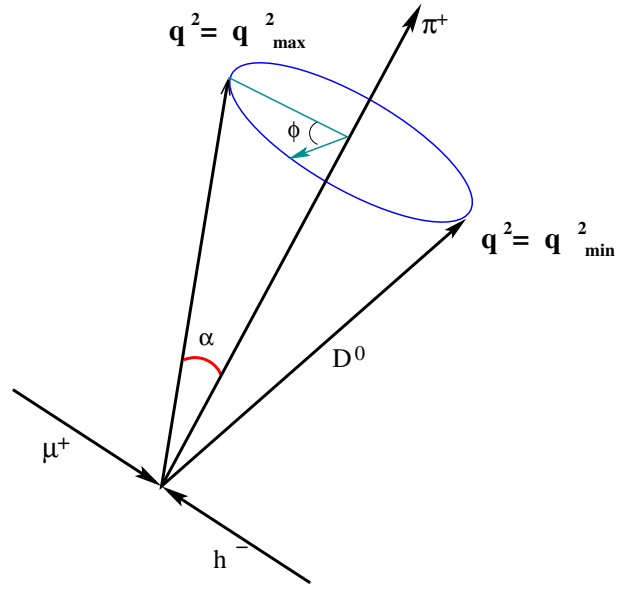
Figure 5.5: The cone closure is obtained by imposing the D^0 mass and the D^* mass in the hadron-lepton rest frame and by choosing the angle \phi corresponding to the D^0 direction that is most consistent with pointing to the primary.
