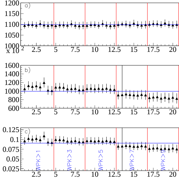
Figure 7.13: Efficiency corrected yields and branching ratio versus piconicity. a) D^0 \rightarrow K^- \mu^+ \nu efficiency corrected yields b) D^0 \rightarrow \pi^- \mu^+ \nu efficiency corrected yields c) Relative branching ratio (in scan of L/\sigma ). For each piconicity cut we scan over eight L/\sigma values. The main source of misidentification in K^- \mu^+ \nu comes from \pi^- \mu^+ \nu decays. The trend on the branching ratio and the \pi^- \mu^+ \nu efficiency corrected yields is consistent with an underestimation of the misidentification rate in the FOCUS Monte Carlo.
