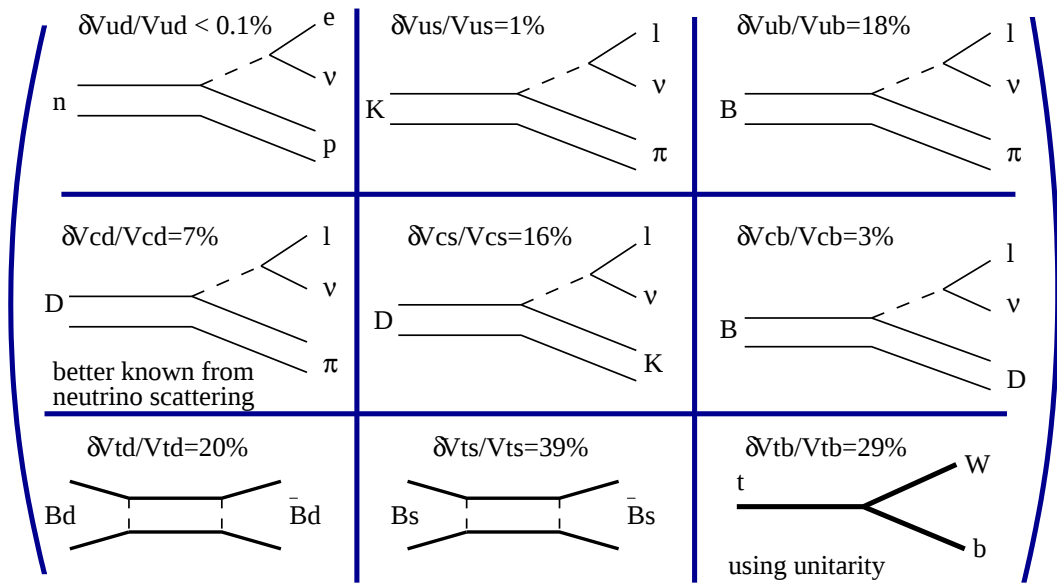
Figure 1.7: The matrix shows the current uncertainties on the CKM matrix elements and the decay modes that have been used to measure them. Semileptonic decays have played an important role in these measurements.
