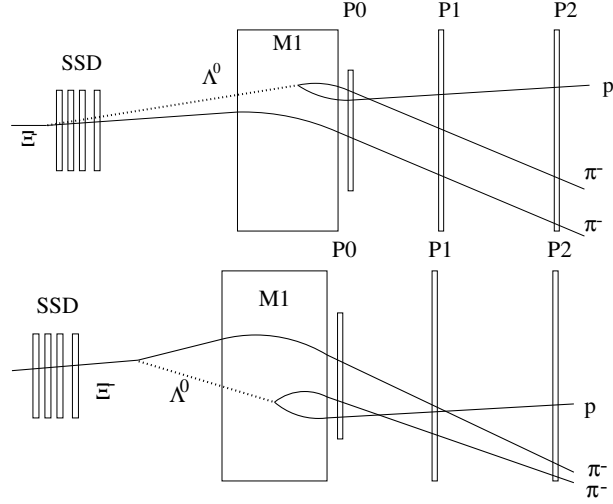
Figure 4.6: A schematic of a \Xi^- decay which occurs upstream (top) and downstream (bottom) of the silicon strip detector (SSD).
