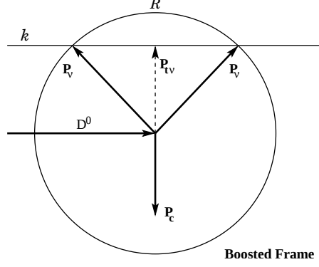
Figure 5.4: Neutrino closure obtained by imposing momentum and energy conservation. From momentum conservation the allowed neutrino momentum lies on the straight line k . From energy conservation the allowed neutrino momenta must lie on the circle \mathcal{R} . The intersections determine the two solutions.
