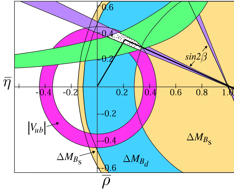
Figure 9.1: Status of the unitary triangle
