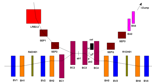
Figure 2: Layout of the upgrade injection system for CSNS-II.
