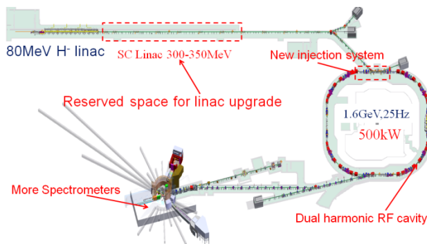
Figure 1: Layout of CSNS-II.
