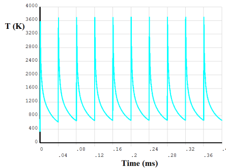
Figure 5: Variation curve of the highest temperature of the main stripping foil in the injection process.
