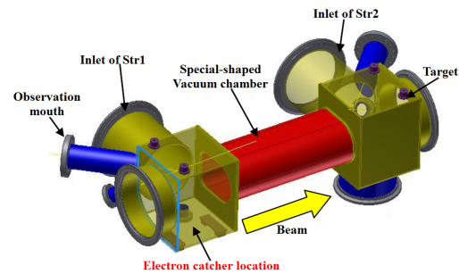
Figure 6: Reserved location for the electron catcher.
