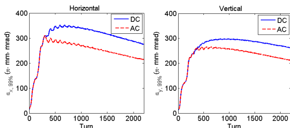
Figure 3: The 99% emittance evolution for the horizontal chicane bump with DC and AC magnets.
