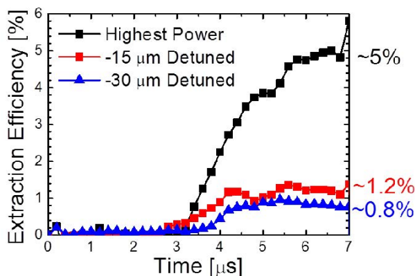
Figure 2: Temporal evolution of extraction efficiency under the relative cavity length of 0, -15 and -30 \mu m. [15]
