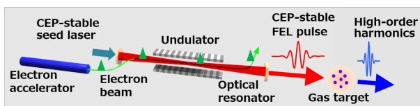
Figure 1: Schematic view of high-harmonics generation driven by an infrared FEL oscillator (FEL-HHG).
