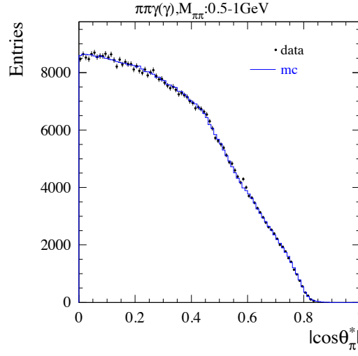
Figure 9.8: The angular pion distribution in the \pi\pi system with respect to the ISR photon direction as function of |\cos\theta_\pi^*| for background-subtracted \pi\pi\gamma(\gamma) data (points) in the \rho central region ( 0.5 < m_{\pi\pi} < 1 GeV) for runs 1-4. The blue histogram is the shape obtained in the simulation, normalized to data.
