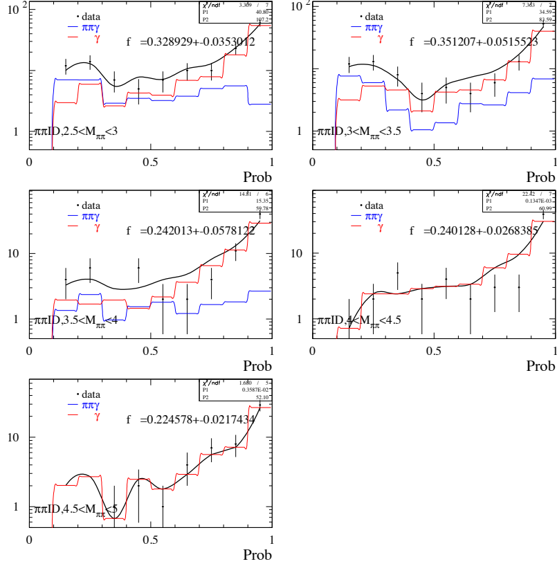
Figure 13.5: The two-component fits of the \pi-\mu probability distributions for '\pi\pi' \rightarrow '\pi_h\pi' events from \mu\mu\gamma and \pi\pi\gamma sources. The \mu\mu fraction in data is expressed in terms of the ratio to the \mu\mu MC sample. Each plot corresponds to a 0.5-GeV mass bin in the range 2.5-5 GeV.
