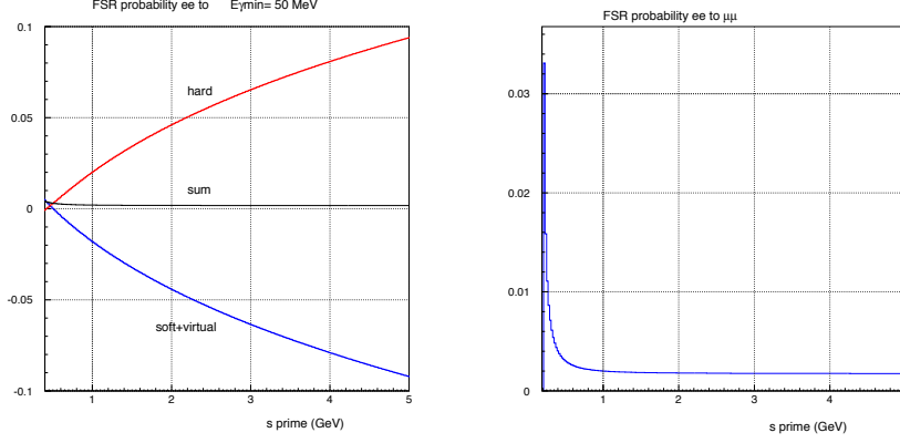
Figure 11.5: The relative FSR contributions as a function of s' in the process e^+e^- \rightarrow \mu^+\mu^-(\gamma_{FSR}) , \frac{\alpha}{\pi}\eta_{h,v+s} at NLO (left), and their sum (right). The separation between hard and soft radiation has been chosen at 50 MeV in the \mu\mu\gamma center-of-mass.
