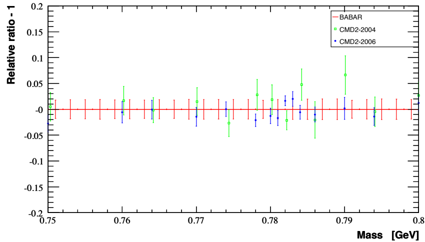
Figure 16.7: The relative difference of form factor squared from the e^+e^- \rightarrow \pi^+\pi^- between BABAR and CMD-2 in the \rho-\omega mass region. Systematic and statistical uncertainties are included for both results, with the diagonal elements of the BABAR covariance matrix.
