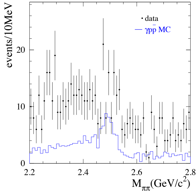
Figure 7.9: The m_{\pi\pi} distribution of data (points) and the p\bar{p}\gamma MC (histogram) reweighted to include the J/\psi \rightarrow p\bar{p} contribution.
