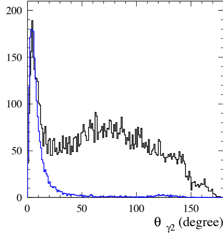
Figure 7.19: The additional 'FSR' photon angular distribution with respect to the closer outgoing muon for the \mu^+\mu^-\gamma(\gamma) events with \ln(\chi^2_{add.FSR} + 1) < \ln(\chi^2_{add.ISR} + 1) , E_{\gamma_{add.FSR}} > 200 MeV and m_{\mu\mu} < 1 GeV (data: black, MC: blue), where MC is normalized to data according to the luminosity.
