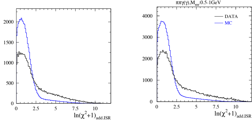
Figure 7.16: The \chi^2_{\text{add.ISR}} distributions of the events with \ln(\chi^2_{\text{add.FSR}}+1) > \ln(\chi^2_{\text{add.ISR}}+1) , E^*_{\gamma_{\text{add.ISR}}} > 200 MeV, m_{\mu\mu} < 1 GeV for \mu^+\mu^-\gamma(\gamma) (left) and 0.5 < m_{\pi\pi} < 1.0 GeV for \pi^+\pi^-\gamma(\gamma) (right), where MC is normalized to data according to the luminosity. (data: black, MC: blue)
