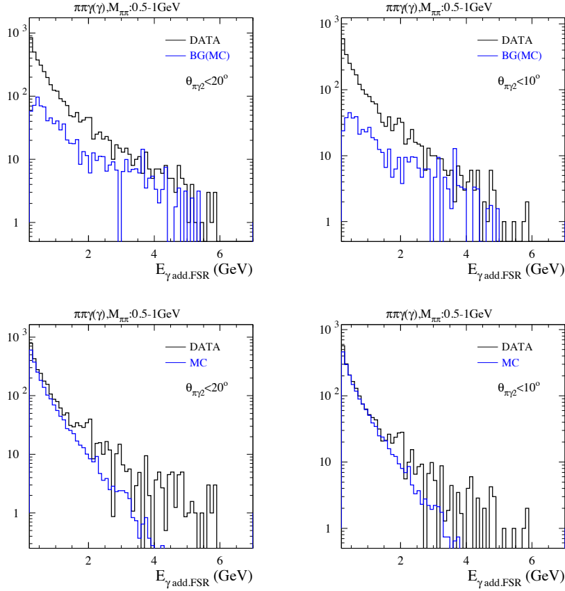
Figure 7.22: The additional FSR photon energy distributions for the \pi\pi\gamma(\gamma) events with \ln(\chi^2_{add.FSR} + 1) < \ln(\chi^2_{add.ISR} + 1) , E_{\gamma_{add.FSR}} > 200 MeV, 0.5 < m_{\pi\pi} < 1 GeV, and \theta_{\pi\gamma_2} < 20^\circ (left), \theta_{\pi\gamma_2} < 10^\circ (right). Top row: data (black), background (blue). Bottom row: background-subtracted data (black), \pi\pi\gamma(\gamma) MC (blue), where MC is normalized to luminosity (there is no large-angle ISR in AfkQed).
