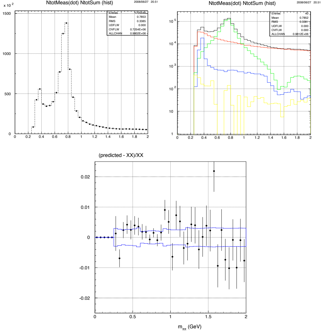
Figure 6.10: The global PID test on data (runs 1-4). Top left: the m_{\pi\pi} spectrum of all XX\gamma events (no PID applied, data points) compared of the sum of identified ' ii ' distributions corrected by the measured ID-efficiencies ((\mu\mu)_0 + (\pi\pi)_0 + (KK)_0 + ee background, histogram). Top right: the different components of the histogram in the top left plot, (\mu\mu)_0 (red), (\pi\pi)_0 (green), (KK)_0 (blue), ee background (yellow), and their sum (black). Bottom: the relative difference of the two spectra in the top left plot (ID-predicted - no PID)/no PID. The deviations are statistically compatible with the estimated systematic uncertainties shown by the blue band.
