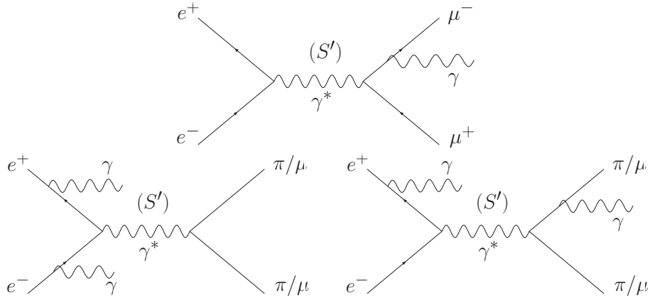
Figure 1.6: Feynman diagrams for the FSR process e^+e^- \rightarrow \gamma\mu^+\mu^- (top), additional ISR process (bottom left) and additional FSR process (bottom right).
