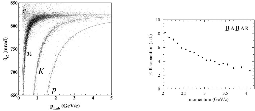
(a) The measured Cherenkov angle \theta_c vs track momentum p_{\text{Lab}} for different charged particles
