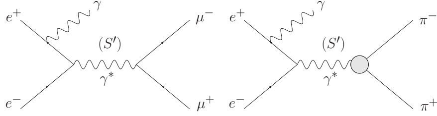
Figure 1.5: Feynman diagrams for the lowest ISR processes e^+e^- \rightarrow \gamma\gamma^* \rightarrow \gamma\mu^+\mu^- (left) and \gamma\pi^+\pi^- (right).
