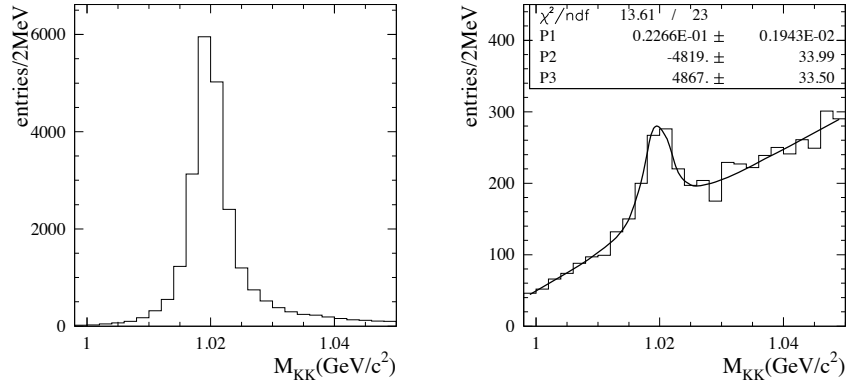
Figure 13.7: Left: the KK mass distribution for KK\gamma MC in the ' \pi_h\pi ' ID sample. Right: the KK mass distribution in the \pi_h\pi ID data sample, fitted with the MC shape (left plot) and a linear component from \pi\pi\gamma (including very small background contributions). The adjustment provides a direct measurement of the KK component in the data sample.
