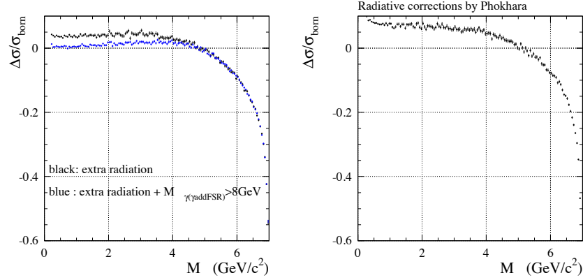
Figure 11.7: The radiative correction C_{rad} defined in Eq. (11.7) for AfkQed (left) and Phokhara (right).
