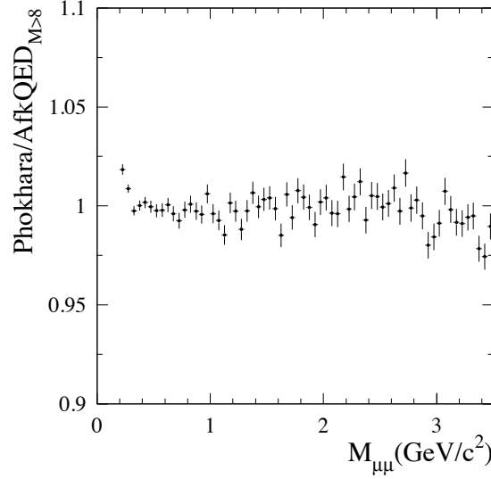
Figure 10.5: The ratio of the \mu\mu mass spectra within acceptance cuts in Phokhara and AfkQEd at generator level with fast simulation.
