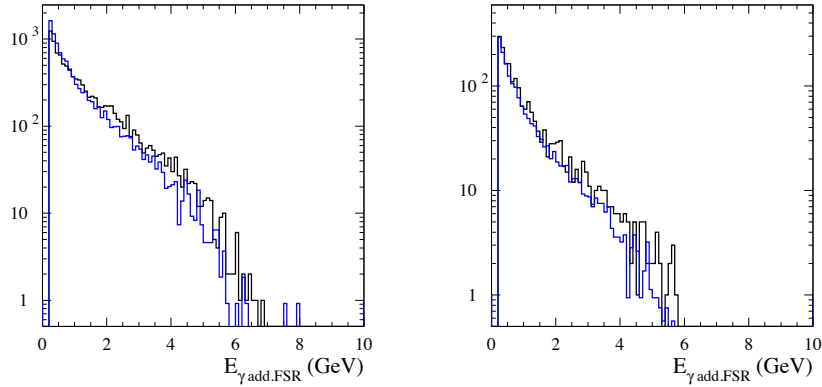
Figure 7.21: Left: The additional 'FSR' photon energy distributions for the \mu^+\mu^-\gamma(\gamma) events with \ln(\chi_{add.FSR}^2 + 1) < \ln(\chi_{add.ISR}^2 + 1) , E_{\gamma add.FSR} > 200 MeV and m_{\mu\mu} < 1 GeV (data: black, MC: blue), where MC is normalized to data according to the number of events (no large-angle ISR in AfkQed). Right: The additional FSR photon energy distributions for the \mu^+\mu^-\gamma(\gamma) events with additional cuts, which are \ln(\chi_{add.FSR}^2 + 1) < 2.5 and \theta_{\mu\gamma 2} < 20^\circ (data: black, MC: blue), here MC is normalized to the BABAR luminosity (runs 1-4).
