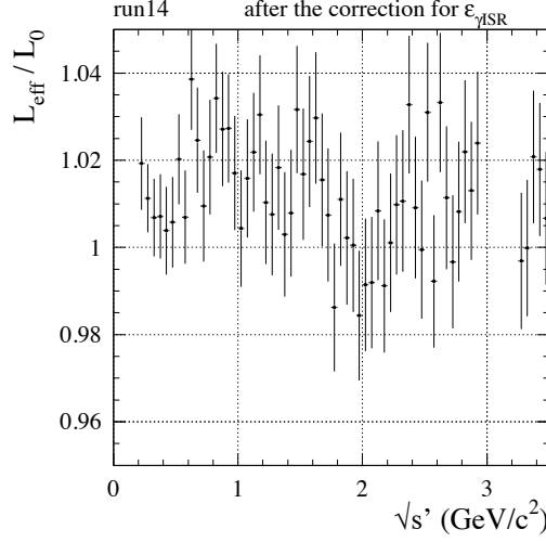
Figure 11.8: The ratio dL_{eff}^{M>8}/dL_{LO} as a function of \sqrt{s'} after correction for the ISR photon efficiency ratio data/MC, i.e. dL_{eff}^{M>8}/dL_{LO} \times \epsilon_{ISR\gamma}^{MC}/\epsilon_{ISR\gamma} .
