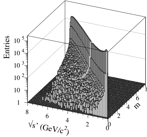
Figure 11.1: The mass transfer matrix from \sqrt{s'} to m_{\mu\mu} from the AfkQed simulation.
