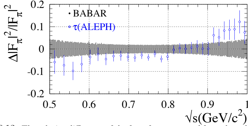
Figure 16.13: The relative difference of the form factor squared from the \tau data of ALEPH with respect to the e^+e^- \rightarrow \pi^+\pi^- BABAR measurements in the 0.5-1 GeV mass region. Systematic and statistical uncertainties are included for both results, with the diagonal elements of the BABAR covariance matrix.
