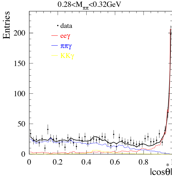
Figure 7.8: The distribution of |\cos\theta^*| of \pi^+\pi^-\gamma events for m_{\pi\pi} < 0.32 GeV after subtraction of \mu^+\mu^-\gamma background and V_{xy} < 0.5 cm (with standard \pi -ID and 2D- \chi^2 cut, runs 1-4). Fit is adjusted with 3 free components: ee from 'RadBhabha' sample (red), \pi\pi\gamma (blue) and KK\gamma (yellow), both from simulation.
