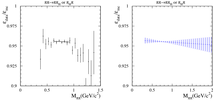
Figure 13.13: Left: The ratio of the efficiency of ' \pi_h \pi ' identification for ' \pi \pi ' identified \pi \pi \gamma(\gamma) events for data and MC, the line is the fitting result (p1) in \rho region. Right: The extrapolation of the ratio fitted in \rho region.
