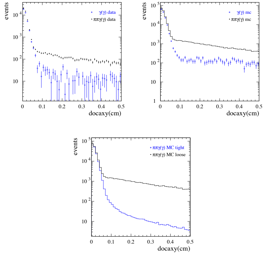
Figure 7.30: Top left: the distribution of the largest of the two transverse distances of closest approach to the interaction point doca_{xy}^{max} for pions and muons in data, for the intermediate \chi^2 region. Top right: the distribution of the largest of the two transverse distances of closest approach to the interaction point doca_{xy}^{max} for pions and muons in simulation, for the intermediate \chi^2 region. Bottom: the distribution of the largest of the two transverse distances of closest approach to the interaction point doca_{xy}^{max} for pions in simulation, for the loose and tight \chi^2 cuts.
