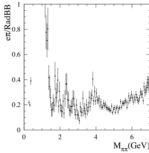
Figure 13.9: The ratio of the mass spectra of ' e\pi ' events and 'RadBhabha' sample. There is a strong contribution from mis-identified \pi\pi events in the \rho region.
