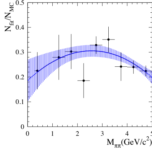
Figure 13.6: The correction factor data/MC for ' \pi\pi ' \rightarrow ' \pi_h\pi ' identification for \mu\mu\gamma , including the luminosity factor ( \sim 0.20 ). The curve with the error band is a second-order polynomial fit to the data points, needed to interpolate in the \rho mass region.
