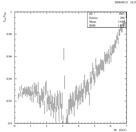
Figure 13.14: The correction for the difference between data and MC on the efficiency of \ln(\chi_{add.ISR}^2 + 1) < 3 cut, which is determined in \mu\mu\gamma(\gamma) data.
