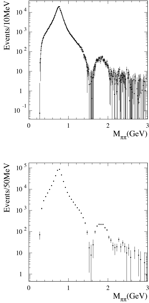
Figure 13.11: The m_{\pi\pi} distribution of \pi\pi\gamma events selected with ' \pi_h\pi ' identification and the tight \ln(\chi^2_{add.ISR} + 1) < 3 cut, from threshold to 3 GeV, in 10-MeV bins (top) and 50-MeV bins (bottom).
