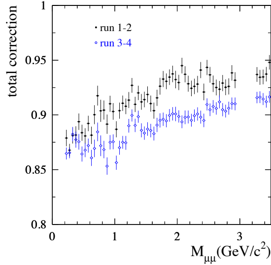
Figure 10.6: The total correction data/MC for the detector simulation as a function of m_{\mu\mu} for runs 1-2 and 3-4.
