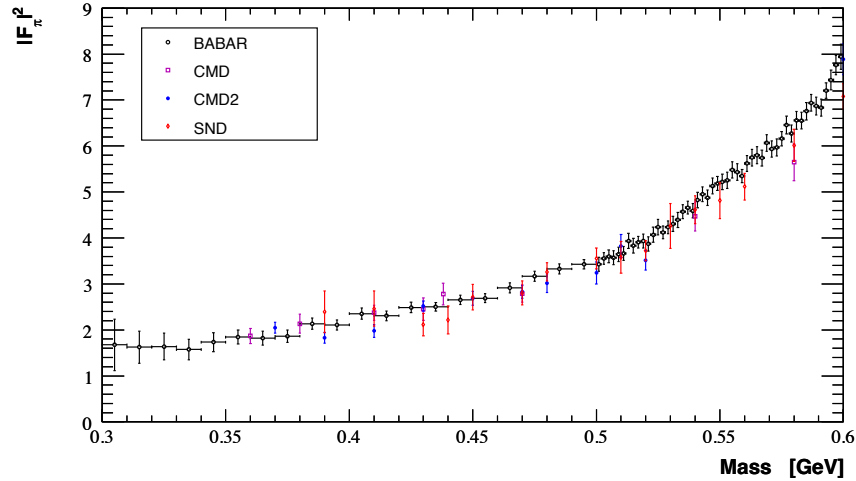
Figure 16.11: The measured pion form factor squared compared to published results from recent experiments. Systematic and statistical uncertainties are shown for all results, with the diagonal elements of the BABAR covariance matrix.
