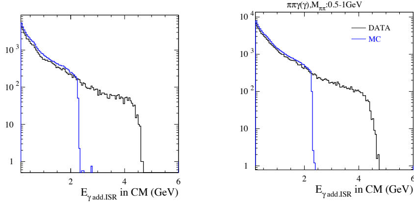
Figure 7.17: The additional ISR photon energy distributions in e^+e^- CM of the events with \ln(\chi^2_{\text{add.FSR}}+1) > \ln(\chi^2_{\text{add.ISR}}+1) , E^*_{\gamma_{\text{add.ISR}}} > 200 MeV, in m_{\mu\mu} < 1 GeV for \mu^+\mu^-\gamma(\gamma) (left) and 0.5 < m_{\pi\pi} < 1.0 GeV for \pi^+\pi^-\gamma(\gamma) (right), where MC is normalized to data according to the luminosity. (data: black, MC: blue)
