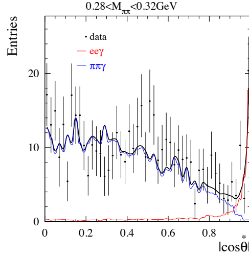
Figure 13.8: The |\cos \theta^*| distribution of ' \pi_h \pi ' data in the 0.28-0.32 GeV m_{\pi\pi} range, fitted (black curve) to two free components: \pi\pi\gamma from MC (blue) and ee background from 'RadBhbha'-flagged events (red). The small \mu\mu\gamma contribution is subtracted out.
