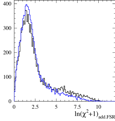
Figure 7.18: The \chi^2_{add.FSR} distributions of \mu^+\mu^-\gamma(\gamma) events with \ln(\chi^2_{add.FSR} + 1) < \ln(\chi^2_{add.ISR} + 1) , E_{\gamma_{add.FSR}} > 200 MeV and m_{\mu\mu} < 1 GeV (data: black, MC: blue), where MC is normalized to data according to the number of events.
