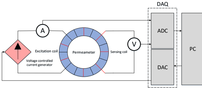
Fig. 1. Architecture of the measurement system [15].
