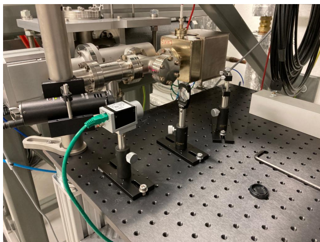
Figure 5: New diagnostic station placed before the beam dump for coherent radiation studies.
