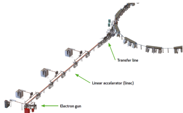
Figure 1: SOLARIS injector LINAC layout.
