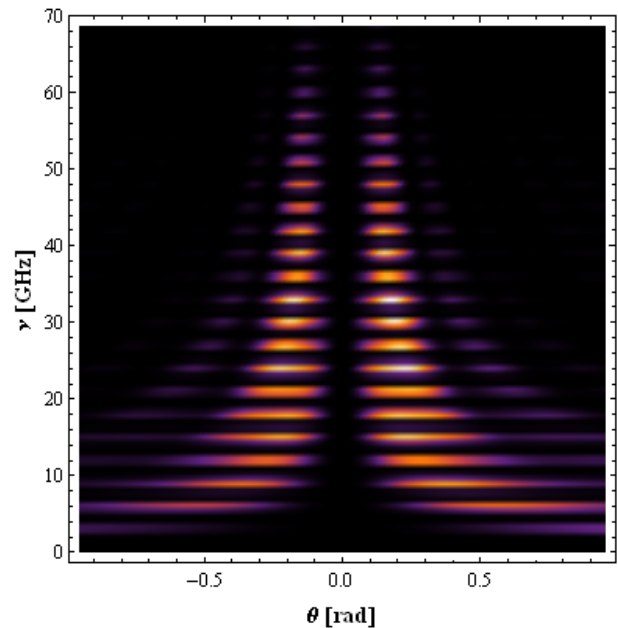
Figure 4: Calculation of the Coherent Diffraction Radiation expected from the bunch profile shown in Fig. 2. The frequency modulation is due to the fact that the time structure of the Solaris bunches is modulated at 3 GHz from the gun. Radiator parameters: 5 cm outer radius, 5 mm inner radius, hollow metallic disk.
