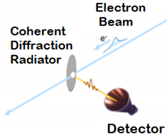
Figure 3: Setup for coherent radiation generation and detection to be adopted for the SOLARIS injector LINAC with the aim to characterize the electron bunch profiles.
