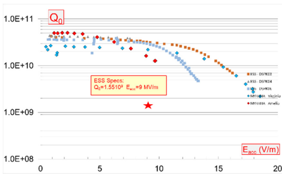
Figure 4: RF performance of ESS and MYRRHA Spoke cavities.
