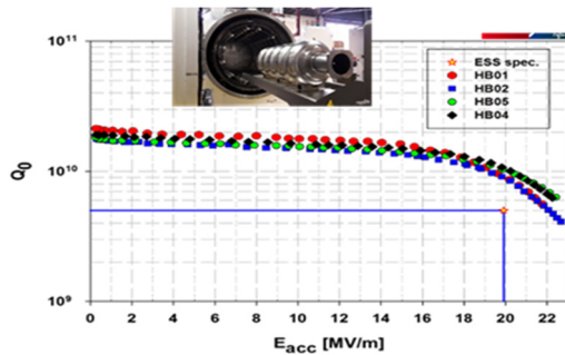
Figure 5: RF characteristics at T=2K of ESS high \beta elliptical cavities developed by CEA Saclay.
