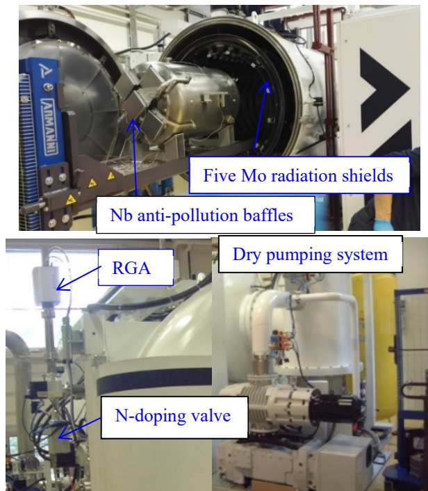
Figure 1: Loading a prototype ESS double-spoke cavity in the furnace.
