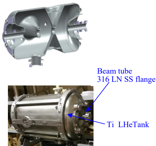
Figure 3: Drawing (A) and photograph (B) of a prototype Double-Spoke cavity for ESS.
