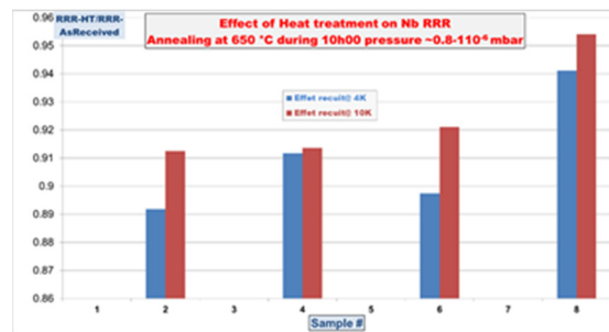
Figure 2: Effect of VH2T2 (10h00 at 650 °C) on Nb RRR.
