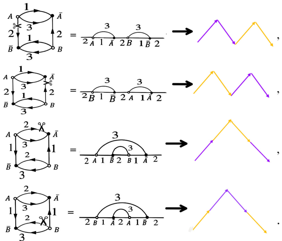
Fig. 9 Correspondence between T_{(id,id,id)}^{(1,0)} , T_{(id,id,id)}^{(0,1)} and length-2 Dyck walks
