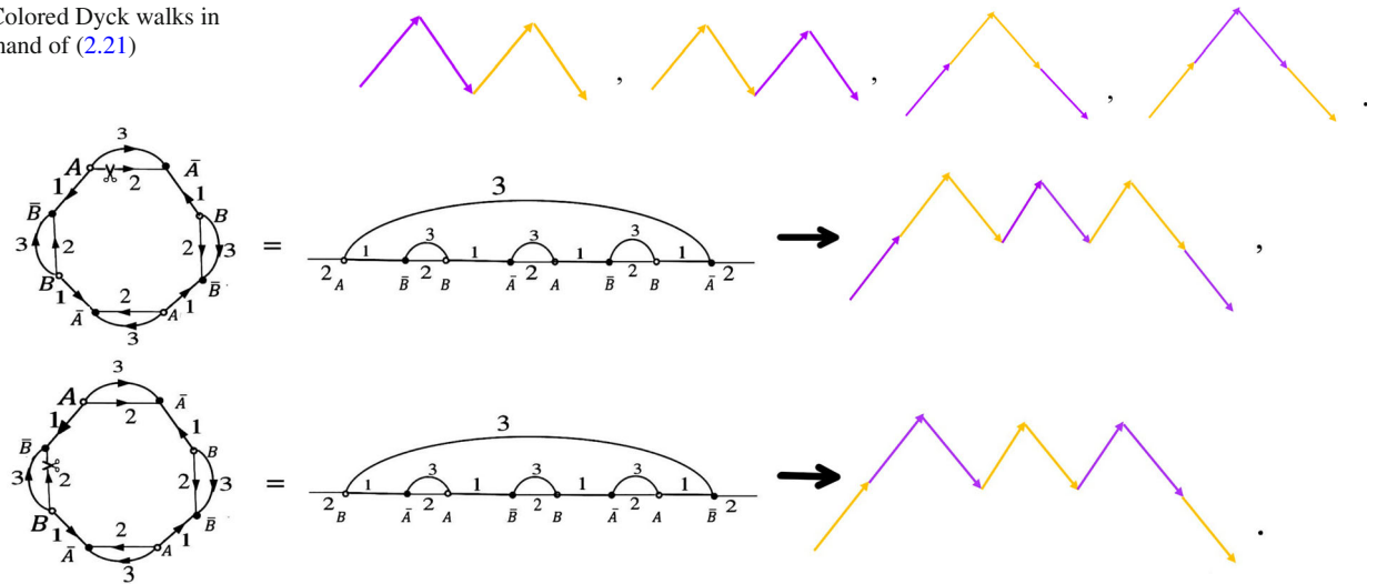
Fig. 8 Correspondence between T_{((1324),id,id)}^{(2,2)} and length-8 Dyck walks
