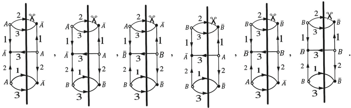
Fig. 13 The cut Feynman diagrams contributing to p_{F,3,3,2}^{(3)}
