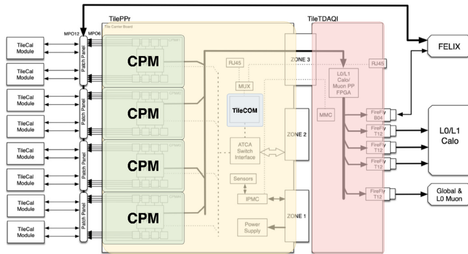
Figure 1. Schematic diagram of the PPr system. A complete PPr system can process the data from eight Tile super-drawers, consists of an ATCA motherboard blade with four CPMs plus one TDAQi RTM [2].
