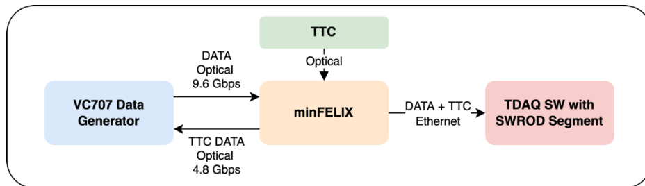
Figure 2. Testbed at the IFIC Laboratory in Valencia composed of front-end boards, Motherboard, Daughterboard and the TilePPr Demonstrator.
