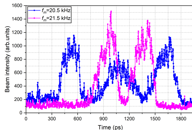
Figure 3: Longitudinal bunch profiles at different modulation frequencies.
