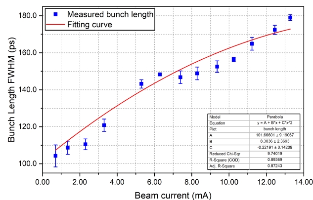
Figure 4: Bunch length via different beam currents.
