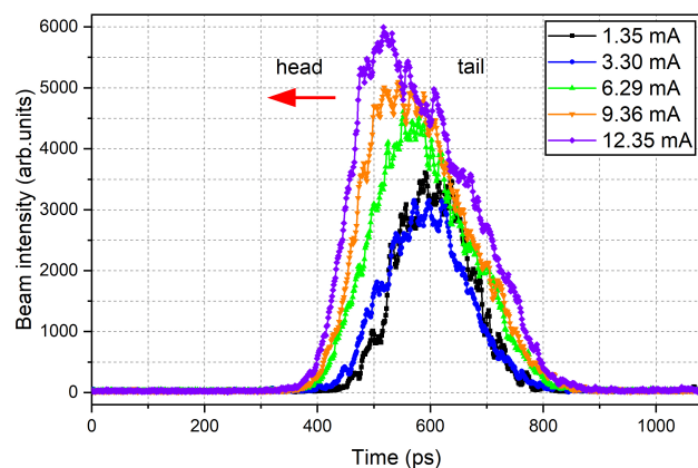
Figure 6: Longitudinal bunch distributions with beam currents.
