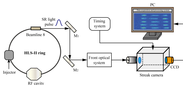
Figure 1: Schematic layout of the streak camera measurement system.
