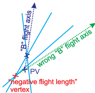
Figure 4. The fit can end up forming a vertex behind the primary interaction vertex, with a negative flight length, which represent a local minimum for the B flight axis direction
