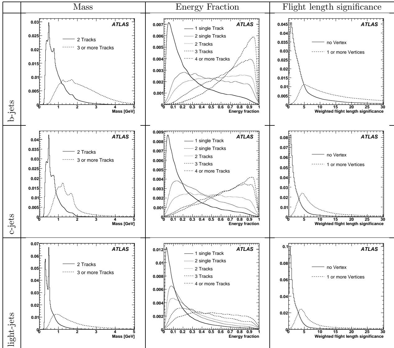
Figure 7. The PDFs for the mass, the energy fraction and the flight length significance are shown, separately for the three different jet-flavours and split according to the decay chain topology found by JetFitter . A vertex is defined here as having at least 2 tracks. Single tracks are considered only in the case no vertex was found.
