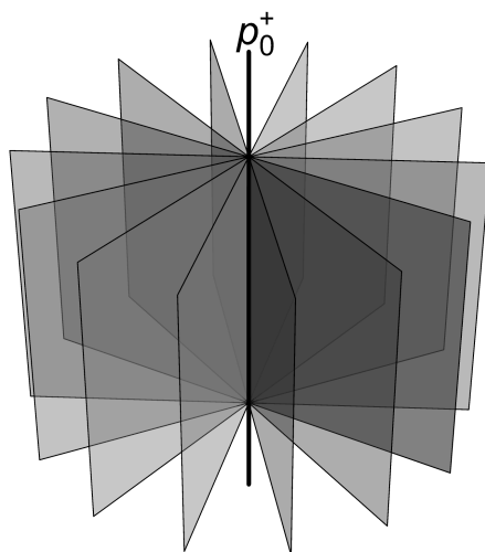
Figure 3. The pencil (sheaf) of light rays through a space–time point.
