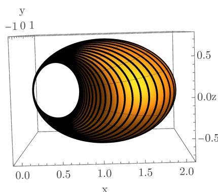
Figure 1. Pictorial representation of the simple conformal infinity with one dimension (coordinate x^3 ) skipped. Parametric plot of the surface defined by Equations (138)–(140), with u \in [0, \pi) , v \in [0, 2\pi) . A needle cyclide made of a one parameter family of null geodesics trapped at infinity.
