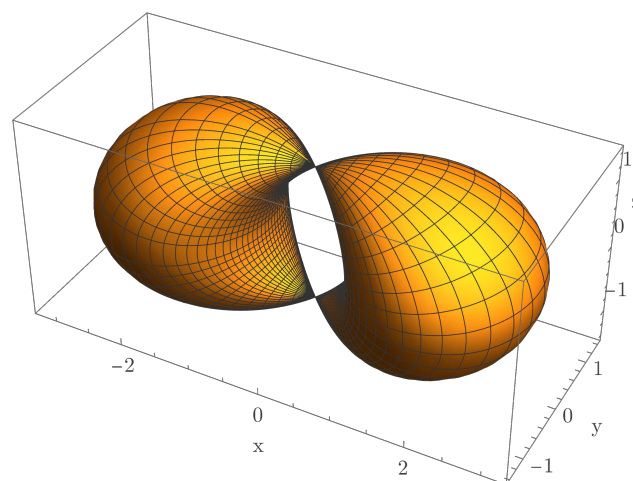
Figure 2. Double cover of the conformal infinity, with space coordinate x^3 suppressed. Parametric plot of the surface defined by Equations (114)–(116), with u, v varying in [-\pi, \pi] , and a = 1.5 . The lines of parameter u connect the two singular points. A squeezed torus, known also as “Horn cyclide” (Cf. [4] (Section 5.4 Cyclides of Dupin, p. 158)).
