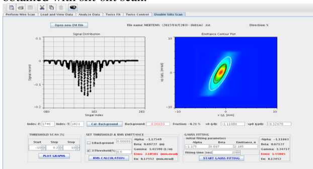
Figure 3: MEBT emittance obtained with slit-slit scan.
