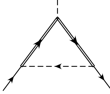
Figure 8.7: One loop \chi b\bar{b} vertex
