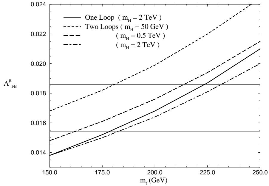
Figure 8.13: Forward-backward asymmetry A_{FB}^\mu (ZFITTER)
