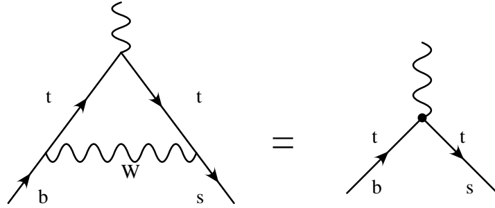
Figure 3.1: b \rightarrow s\gamma process in SM
