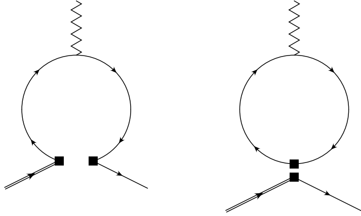
Figure 5.4: Mixing of 4-fermion operators with \bar{O}_{1\dots 8}^+ operators.
