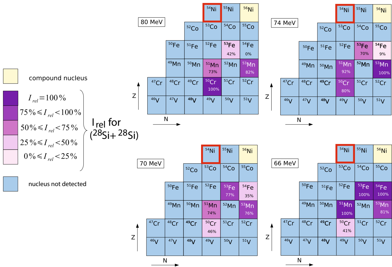
Fig. 4 Part of the table of isotopes with the products of fusion–evaporation reactions formed by the symmetric beam and target combination ^{28}\text{Si} + ^{28}\text{Si} . The colour depth is chosen with respect to the yields of the transitions in Table 1
