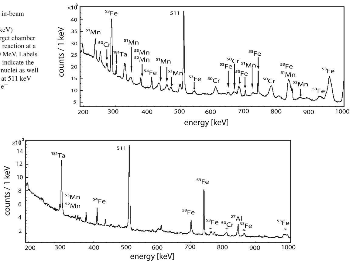
Fig. 6 Part of the \gamma -ray spectrum ( E_\gamma = 200 –1000 keV) at the ‘CD chamber’. The spectrum is dominated by \gamma -ray transitions from known isomers populated in the ^{28}\text{Si} + ^{28}\text{Si} reaction at a beam energy of 70 MeV. The broad peaks, which are marked with asterisks (*) are caused by intense \gamma -ray transitions from prompt events at the target
