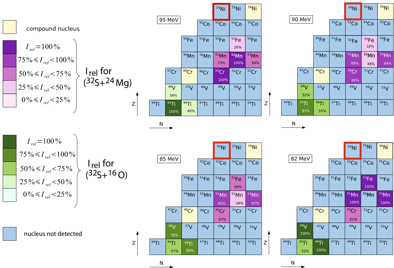
Fig. 3 Part of the table of isotopes with the identified reaction products following the fusion–evaporation reactions ^{32}\text{S} + ^{24}\text{Mg} and also between beam particles and oxygen contaminants on the surface of the
