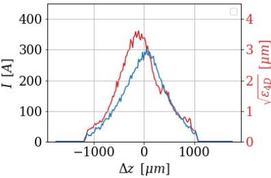
Figure 2: Current profile and slice emittance in 1-nC case.
