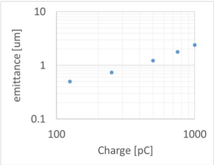
Figure 6: Emittance vs bunch charge.
