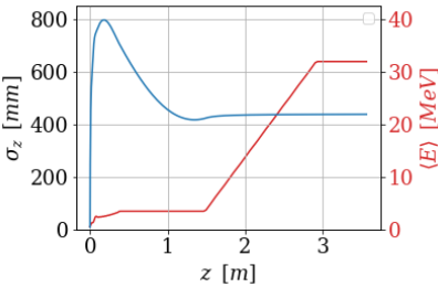
Figure 5: Bunch length and energy along Z in 1-nC case.
