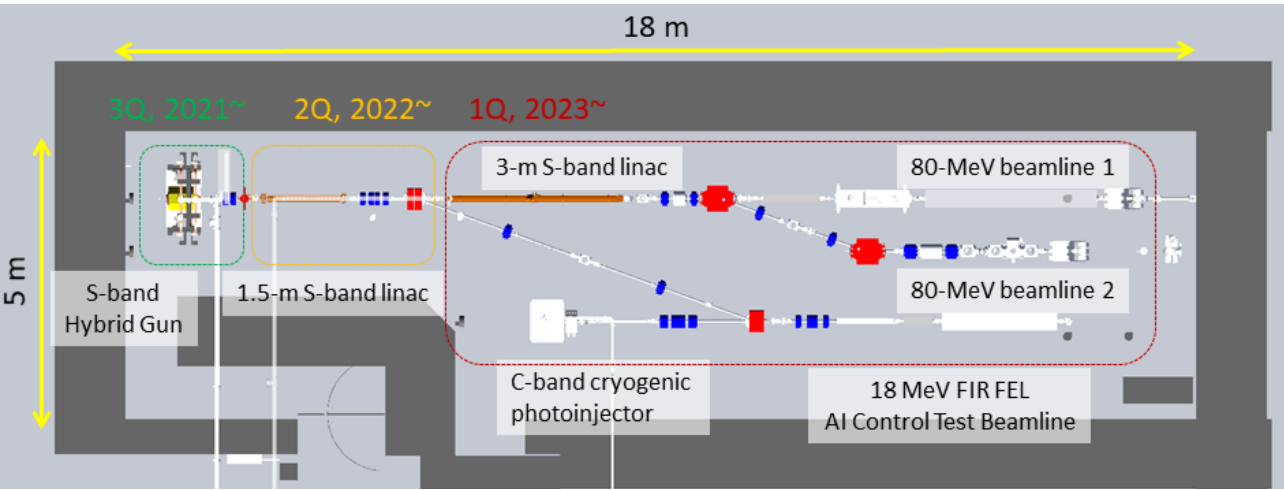
Figure 1: Layout of SAMURAI bunker.
