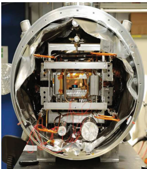
Figure 1: The SIS100 dipole
