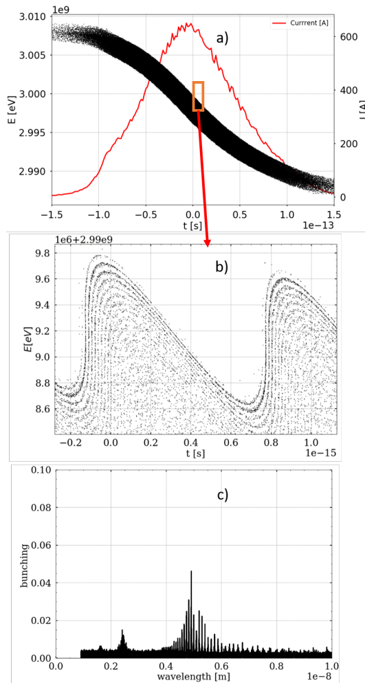
Figure 3: a) Longitudinal phase space (black) and current (red). b) Zoomed in phase space after Chicane 2 with CSR on and with the mitigated beam. c) Bunching vs. wavelength for the mitigated beam with CSR on at the end of Chicane 2.
