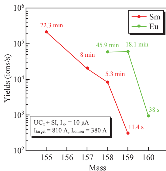
Figure 5. Yields measured for Sm and Eu isotopes released by \text{UC}_x pellets during the on-line experiment performed with the SI ion source.
