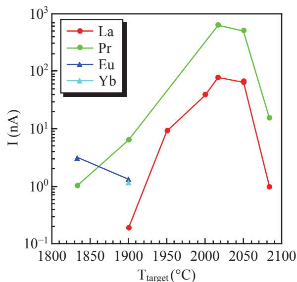
Figure 4. Ion beam intensity measured during the on-line experiment performed with the SI ion source for La, Pr, Eu and Yb stable isotopes released by \text{UC}_x pellets without \text{CF}_4 .
