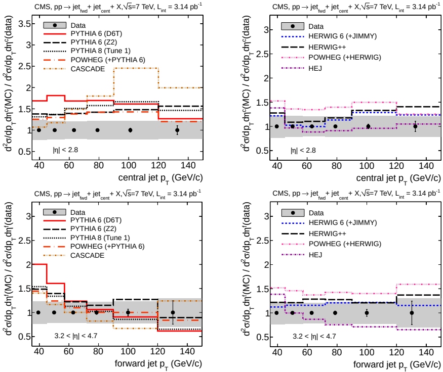
Fig. 4. Ratios of theory predictions to data for distributions presented in Fig. 3.
