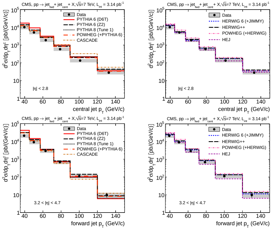
Fig. 3. Results of the measurement of inclusive cross-section for the production of a forward jet associated with a central jet as a function of the central jet p_T (top plots) or the forward jet p_T (bottom plots). Results for the data are compared to PYTHIA6, PYTHIA8, POWHEG (+PYTHIA), CASCADE predictions (left) and to HERWIG6, Herwig++, POWHEG (+Herwig), HEJ predictions (right).
