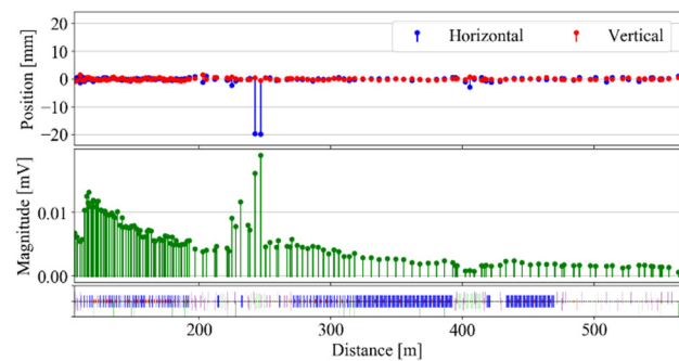
Figure 5: BPM readings along the linac after the completion of the ^{86}\text{Kr}^{34+} beam steering correction. The large signals from the FS1 BPMs is related to the fact that the 180° bend was intentionally tuned for charge state 33.5+.
