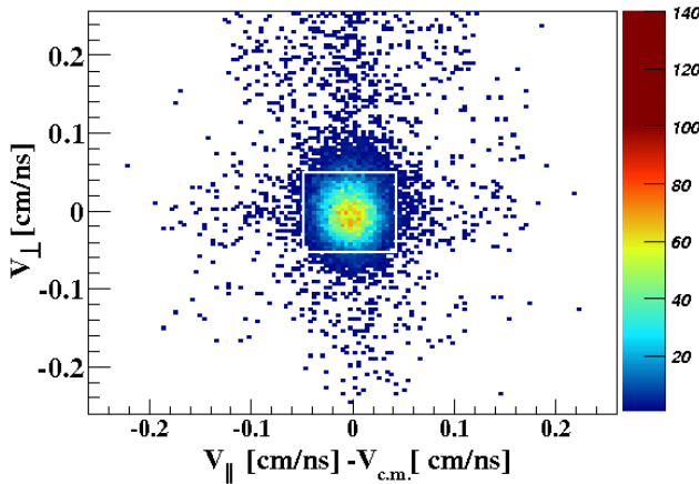
Fig. 1. Measured distribution of velocity components of FF at beam energy of 89 MeV for the reaction ^{19}\text{F} + ^{206}\text{Pb} \rightarrow ^{225}\text{Pa}^* . Full momentum transfer fission events are shown inside white rectangular box and transfer fission events are lying around this rectangular box.
