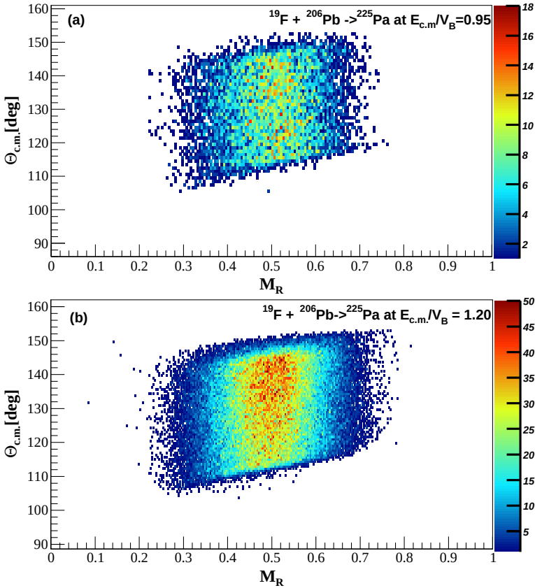
Fig. 2. FF mass-angle correlations for reactions ^{19}\text{F} + ^{206}\text{Pb} \rightarrow ^{225}\text{Pa}^* at (a) 5% below the fusion barrier and (b) 20% above the fusion barrier. No mass-angle correlation for ^{225}\text{Pa} nuclei are observed around barrier energies.
