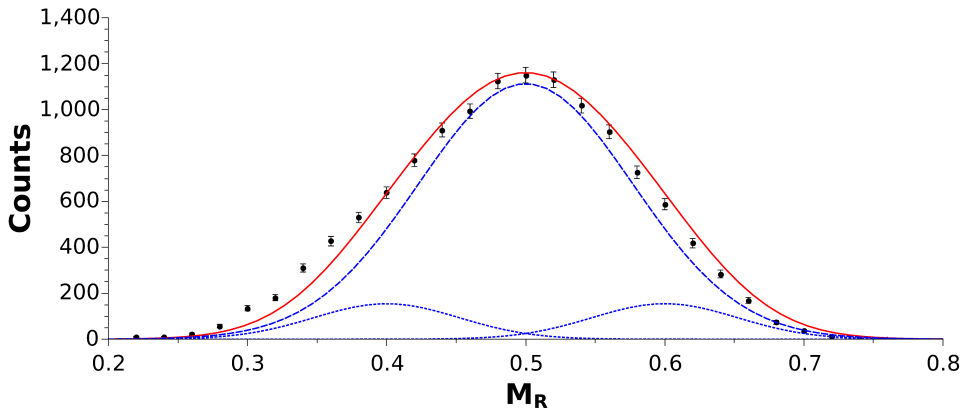
Fig. 3. Measured mass ratio ( M_R ) distribution of fission fragments for the reaction ^{19}\text{F} + ^{206}\text{Pb} \rightarrow ^{225}\text{Pa}^* at E_X = 31.8 MeV energy. Gaussian fitted with solid (red) line is the sum of all three dotted (blue) Gaussians. Their M_R peak positions are lying around 0.5 (larger Gaussian), 0.41 (left Gaussian — centroid of light fragment mass around 93), 0.59 (right Gaussian — centroid of the heavy fragment mass around 132), respectively.
