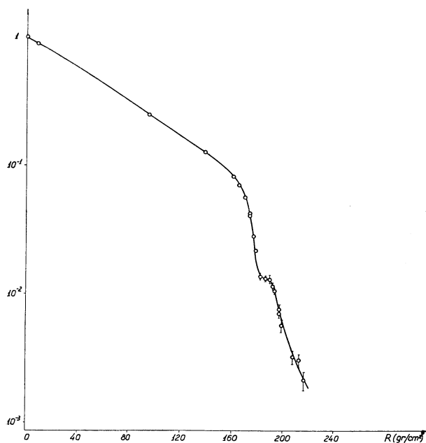
Fig. 3. A typical integral range curve ( E_{\pi} = 307 Mev).
