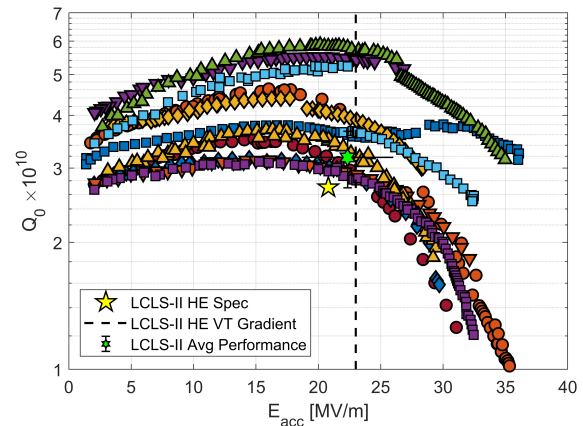
Figure 3: Q_0 vs E_{acc} performance for single-cell cavities treated with the 3/60 recipe. Excellent performance was achieved, with some Q_0 as high as 6 \times 10^{10} at 2 K.
