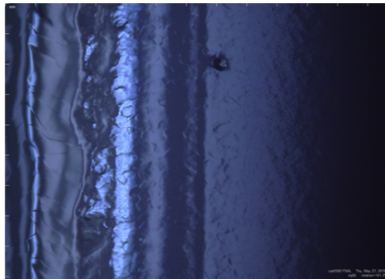
Figure 7: An example optical inspection issue from one of the 16 cavities produced by EZ. The weld appears wavy and a defect is present, suggesting an improper weld stackup prior to electron-beam welding.
