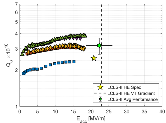
Figure 5: Q_0 vs E_{acc} performance of the 9-cell cavities treated with the 3/60 recipe.
