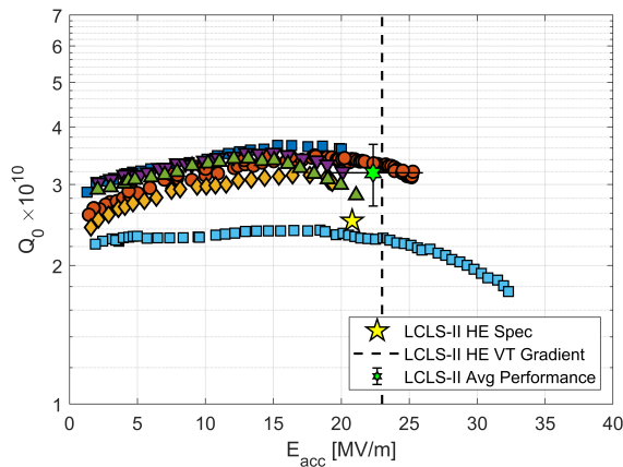
Figure 4: Q_0 vs E_{acc} performance of the 9-cell cavities treated with the 2/0 recipe.
