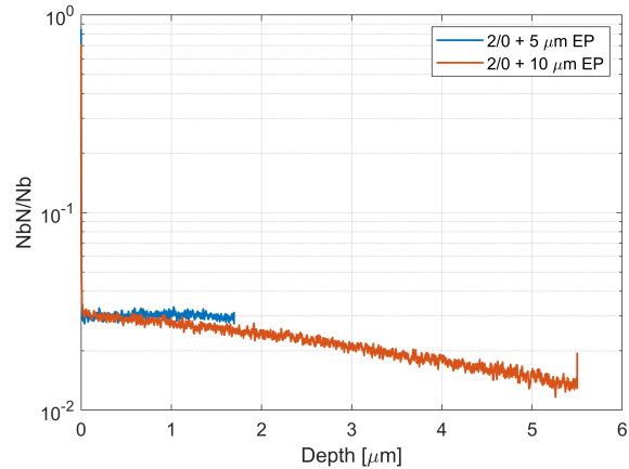
Figure 10: SIMS data taken at FNAL on a sample doped in the FNAL furnace with the 2/0 doping.
