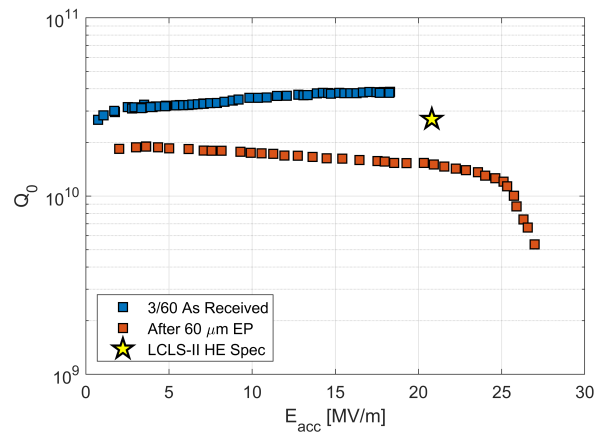
Figure 8: Q_0 vs E_{\text{acc}} performance of a cavity treated with 3/60 at the vendor and then reset with 60 \mu\text{m} EP at FNAL. After reset, the cavity performs similar to standard prepared cavities, suggesting that manufacturing issues were not present.
