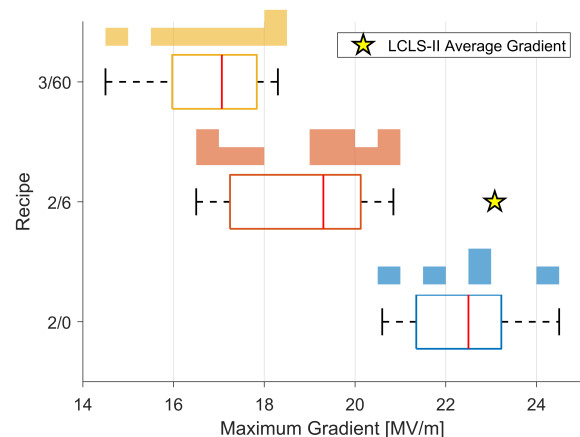
Figure 6: A comparison of the quench fields for 9-cell cavities prepared with the three different recipes at the cavity vendors. 2/6 Baseline performance was significantly worse than the average LCLS-II performance. The 2/0 recipe demonstrated an average increase of 3 MV/m with respect to the 2/6 recipe. The colored bars show histograms of the results, overlaid with the boxplot. The scale for each of the histograms are the same.
