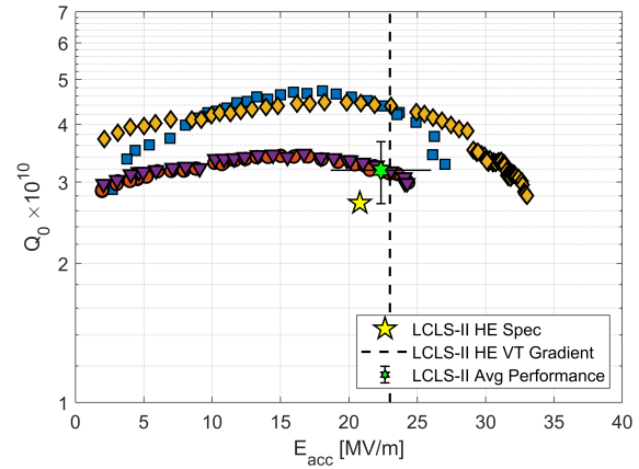
Figure 2: Q_0 vs E_{acc} results for single-cell cavities prepared with the 2/0 recipe. Also, shown is the average LCLS-II cavity performance. All single-cell cavities prepared exceed the LCLS-II HE specification.
