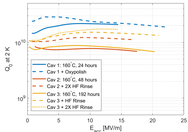
Figure 1: Q_0 vs E_{acc} performance for the three cavities prepared with nitrogen-infusion at Cornell. Contamination in the furnace led to high residual resistance which limited the Q_0 .
