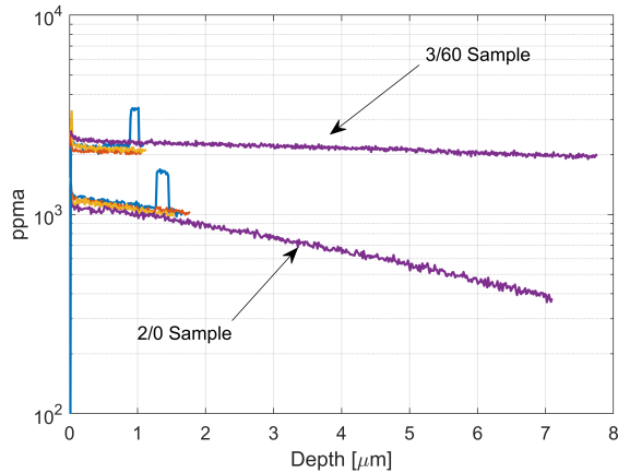
Figure 9: SIMS data showing the depth profile of 3/60 and 2/0 samples treated in RI's furnace with the 9-cell cavities. 0 \mu\text{m} of depth on this plot is after a 5 \mu\text{m} EP. Colors represent different locations on the sample measured.
