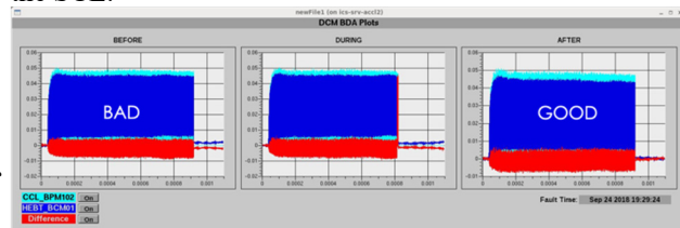
Figure 4: Example of the SCL DCM data storage from the initial installation. The first set of waveforms are before errant beam, middle during, and on the right after the event. All show beam current during the beam pulse.
