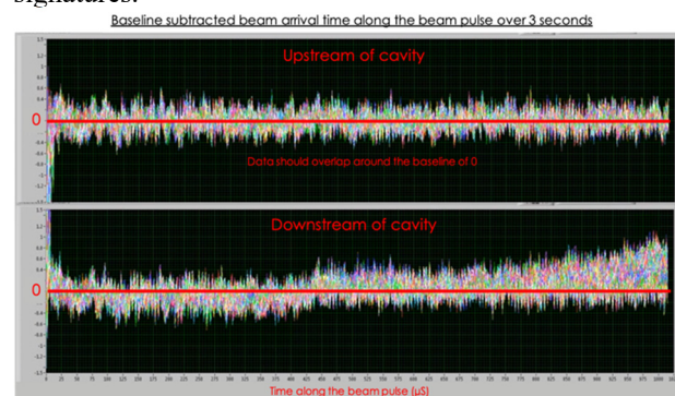
Figure 5: Example of the BPM phase data during the beam pulse. The top is just upstream of a set of SRF cavities and the bottom just downstream of the same set of SRF cavities. The different colors are 180 different beam pulses. Downstream of the cavities the phase slews enough to be seen by eye. This event caused a beam trip.
