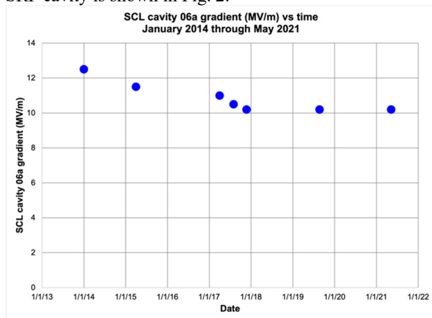
Figure 2: SRF cavity 06a field has been lowered from 12.5 MV/m to 10.2 MV/m over the last 7 years. The field has stabilized since installing a new interlocking scheme in 2018.
