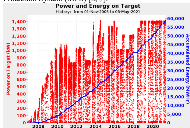
Figure 1: Beam power ramp up history at SNS.
