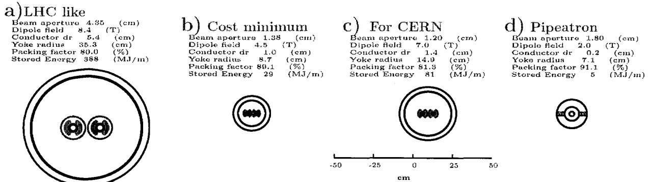
FIG. 2: Comparative Cross sections: a) LHC like: high field, large aperture; b) Proposed: low field, small aperture; c) For CERN: higher field small aperture; d) Pipeatron: very low field, small aperture.
