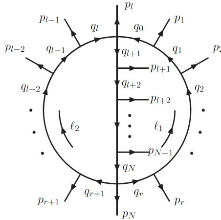
Fig. 2. Momentum configuration of the two-loop N -point scalar integral.
