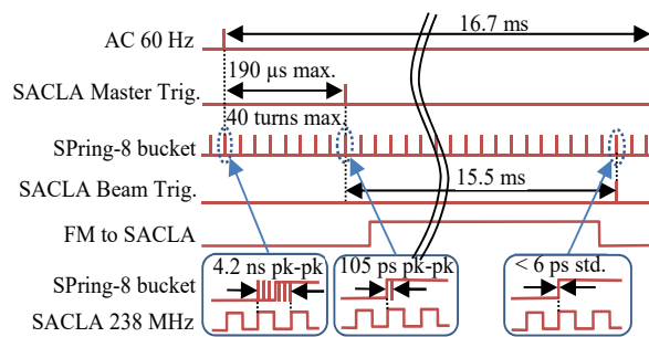
Figure 3: Timing chart of the synchronization system.
