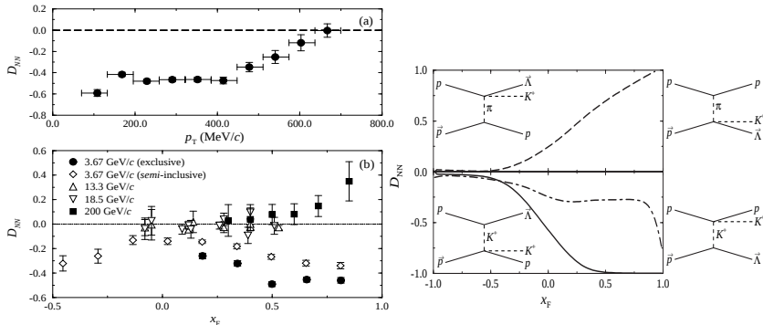
Fig. 4. left:(a) Measured D_{NN} values vs. transverse momentum transfer for the exclusive pK^+\Lambda reaction. (b) D_{NN} as a function of x_F for the present exclusive \Lambda production and for inclusive \Lambda production at various higher incident momenta from Refs. [32, 33]. Also shown for comparison are the semi -inclusive results from the present data. right:Theoretical calculation [1] of D_{NN} for various exclusive \Lambda production mechanisms: kaon-exchange (solid curve), pion-exchange (dashed), or both combined with a \Lambda - p final state interaction (dot-dashed). The Feynman diagrams indicate the dominant exchange contributions for positive vs. negative x_F . The calculations are integrated over all phase space in other kinematic variables.
