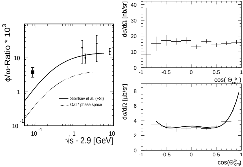
Fig. 2. (left) Ratio of the exclusive total cross sections for the pp\phi and pp\omega reactions as a function of the available energy above the \phi production threshold. Shown is the value measured in this work (square) together with data at higher energies (dots) and model calculations described in the text. (right) Angular distribution of the \phi and \omega mesons (top and bottom, respectively). The error bars indicate only the statistical errors and for the \omega meson the curve shows a fit with the sum of even Legendre polynomials.
