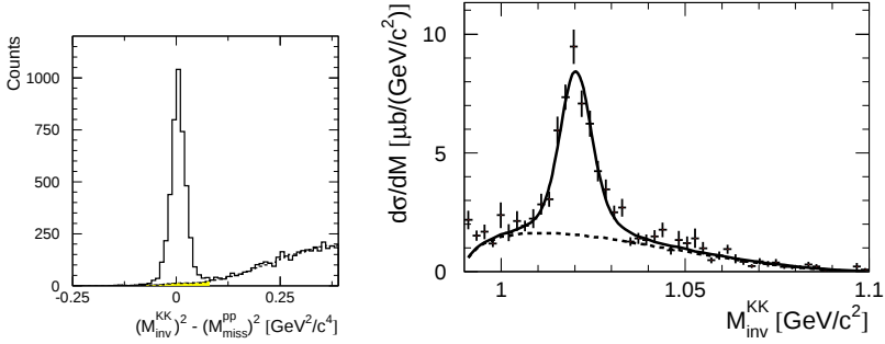
Fig. 1. (left) Spectrum of (M_{\text{inv}}^{KK})^2 - (M_{\text{miss}}^{pp})^2 . The solid histogram is for events with kaon identification and the dashed histogram is the scaled background determined from events without kaon identification. (right) Acceptance corrected M_{\text{inv}}^{KK} distribution. The dashed curve is an estimate of the non-resonant contribution. The solid curve is the sum of the non-resonant and the \phi meson contribution.
