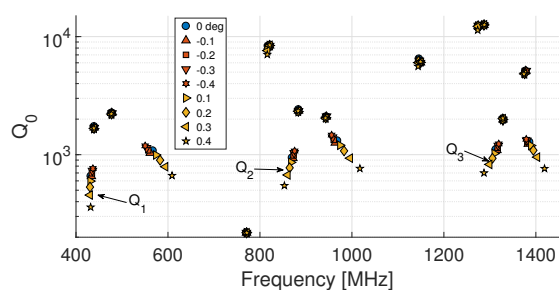
Figure 7: Quality factor vs. Frequency of the QPR at room temperature with a rotation of the rods around the y -axis with an angle \theta between -0.4^\circ and 0.4^\circ .
