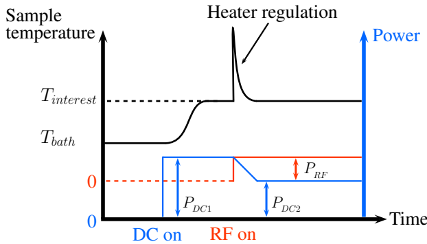
Figure 3: Illustration of the calorimetric measurement principle [2].
