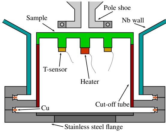
Figure 2: Cross-sectional view of the calorimetry chamber.
