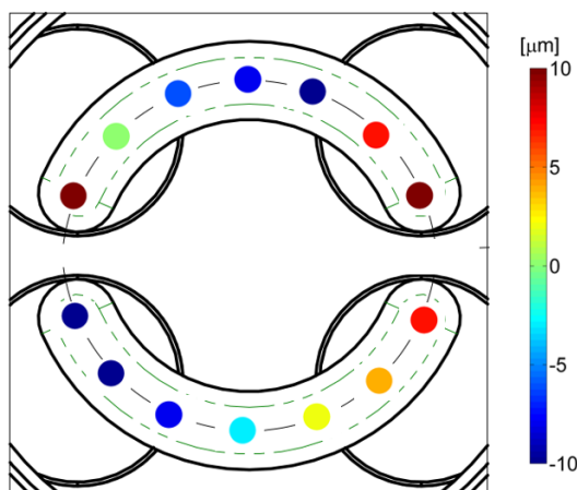
Figure 5: Parallelism of the pole shoes measured at Zanon Research & Innovation Srl. The deviations with respect to the nominal plane are within our tolerance values.
