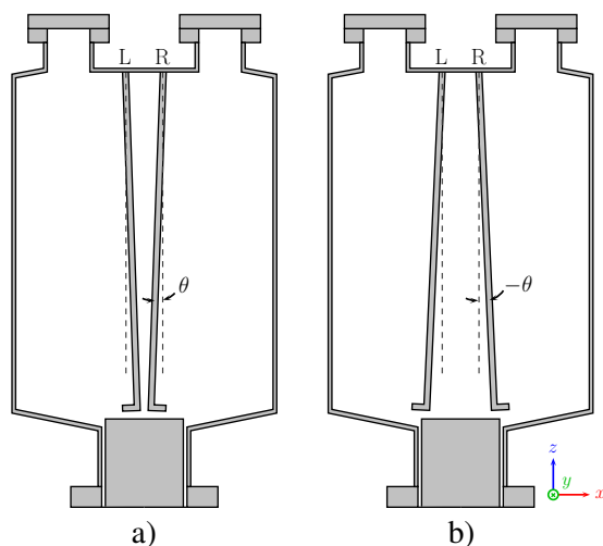
Figure 6: Schematic diagram of the angle variation of the Nb rods. The rotation of the rods was done around the y -axis with an angle \theta that is a) positive when the rods get closer and b) negative when the rods draw apart.
