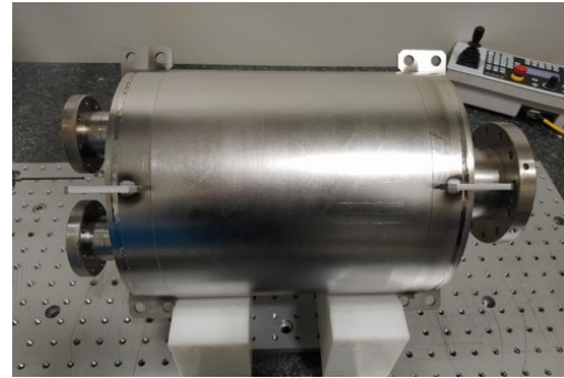
Figure 4: Finalized QPR at Zanon Research & Innovation Srl.
