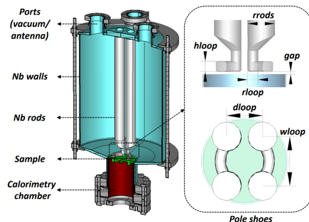
Figure 1: Cross-sectional view of a QPR (left) with the parametrized model of the pole shoes (right) [2].
